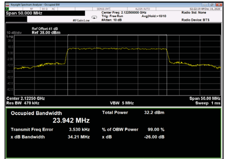
Figure 768: QPSK 25MHz B.W.; 2122.5MHz, 15kHz - Output
