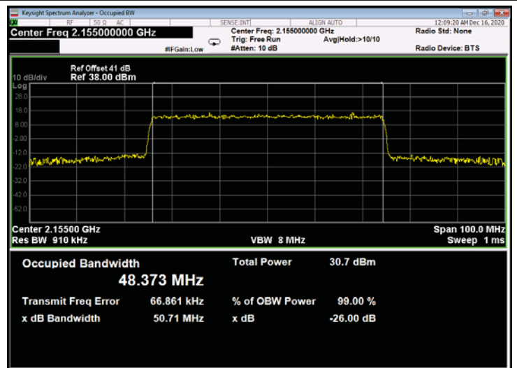
Figure 660: 64QAM 50MHz B.W.; 2155.0MHz, 15kHz - Output
