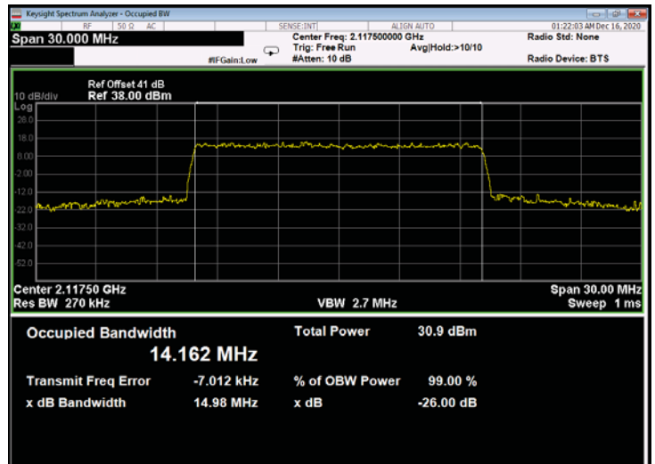
Figure 684: 256QAM 15MHz B.W.; 2117.5MHz, 15kHz - Output
