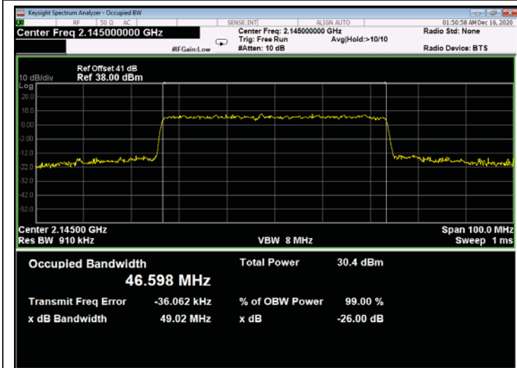
Figure 725: 256QAM 50MHz B.W.; 2145.0MHz, 60kHz - Output
