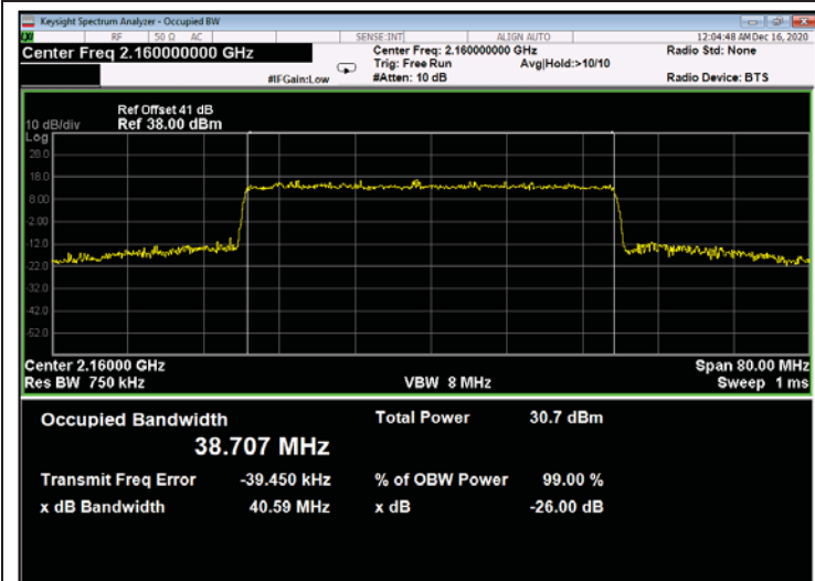
Figure 651: 64QAM 40MHz B.W.; 2160.0MHz, 15kHz - Output
