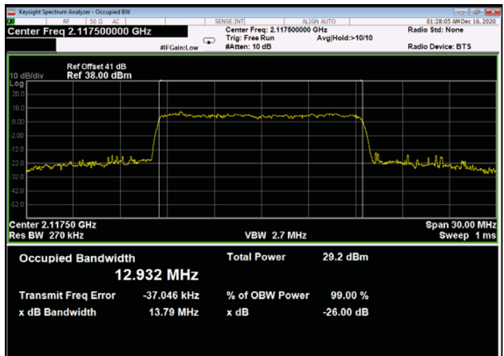
Figure 686: 256QAM 15MHz B.W.; 2117.5MHz, 60kHz - Output
