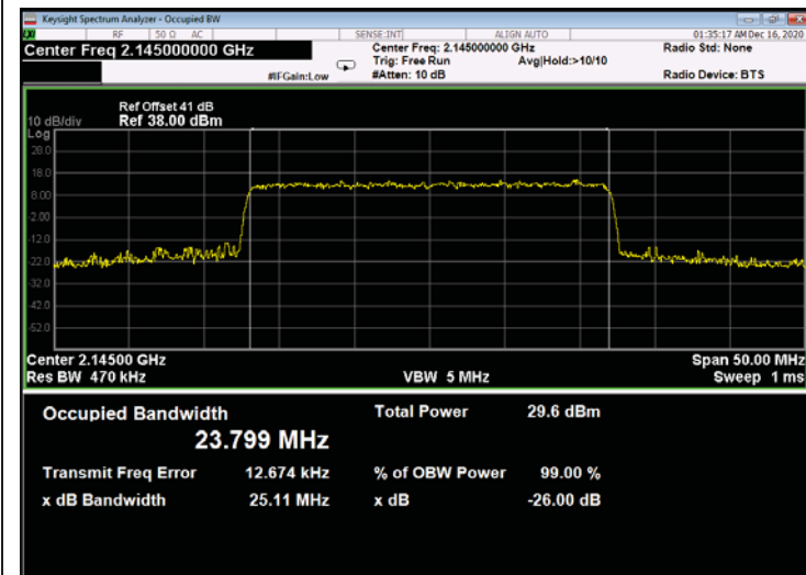
Figure 705: 256QAM 25MHz B.W.; 2145.0MHz, 15kHz - Output
