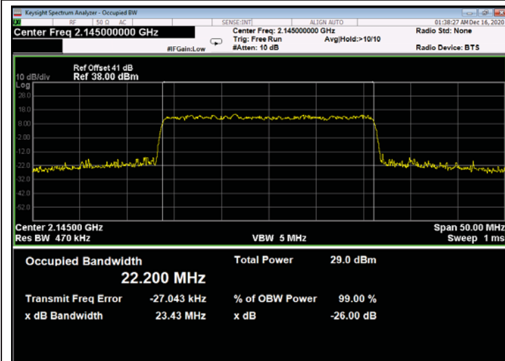
Figure 707: 256QAM 25MHz B.W.; 2145.0MHz, 60kHz - Output
