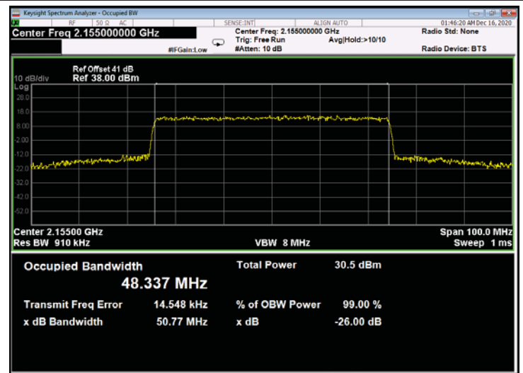
Figure 726: 256QAM 50MHz B.W.; 2155.0MHz, 15kHz - Output
