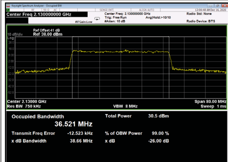
Figure 647: 64QAM 40MHz B.W.; 2130.0MHz, 60kHz - Output
