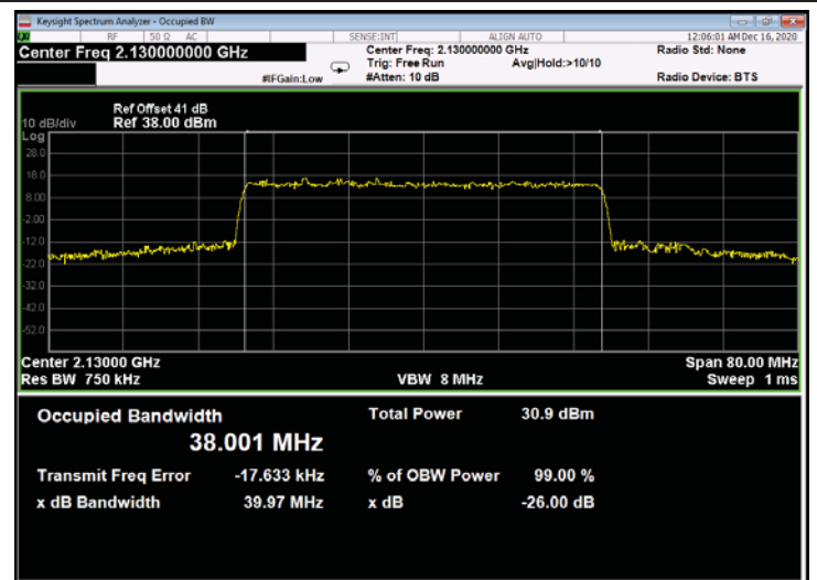
Figure 646: 64QAM 40MHz B.W.; 2130.0MHz, 30kHz - Output
