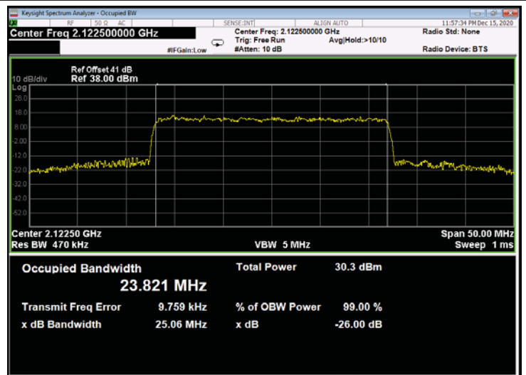
Figure 636: 64QAM 25MHz B.W.; 2122.5MHz, 15kHz - Output
