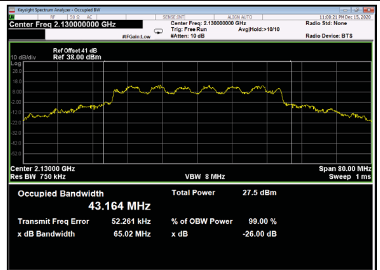
Figure 580: 16QAM 40MHz B.W.; 2130.0MHz, 30kHz - Output
