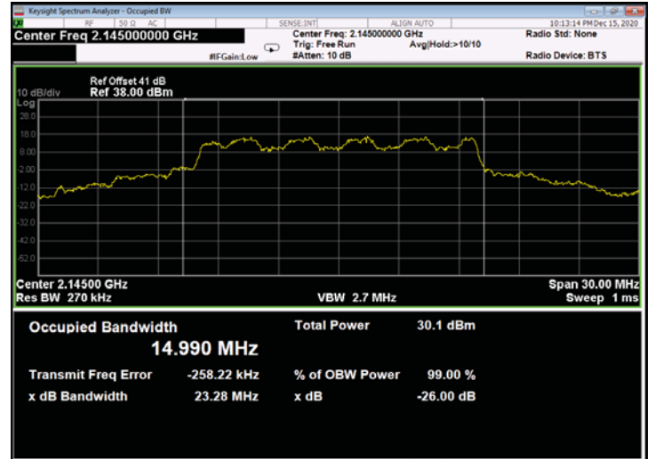
Figure 556: 16QAM 15MHz B.W.; 2145.0MHz, 30kHz - Output
