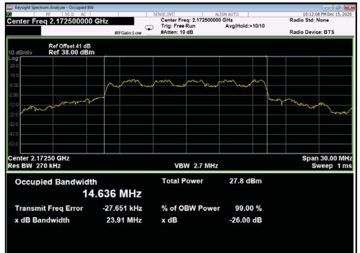
Figure 558: 16QAM 15MHz B.W.; 2172.5MHz, 15kHz - Output
