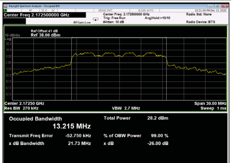
Figure 560: 16QAM 15MHz B.W.; 2172.5MHz, 60kHz - Output
