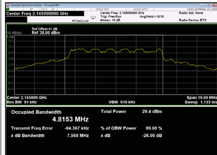
Figure 539: 16QAM 5MHz B.W.; 2145.0MHz, 15kHz - Output
