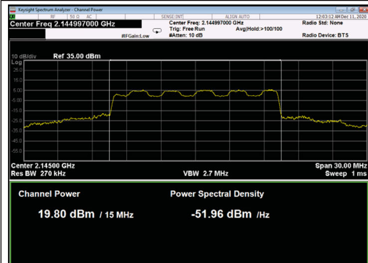
Figure 27: 16QAM 15MHz B.W.; 2145.0MHz, 15kHz
