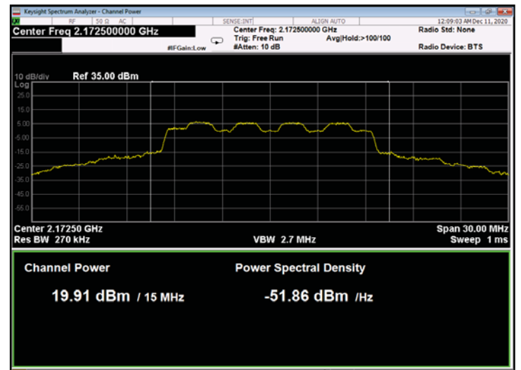
Figure 32: 16QAM 15MHz B.W.; 2172.5MHz, 60kHz
