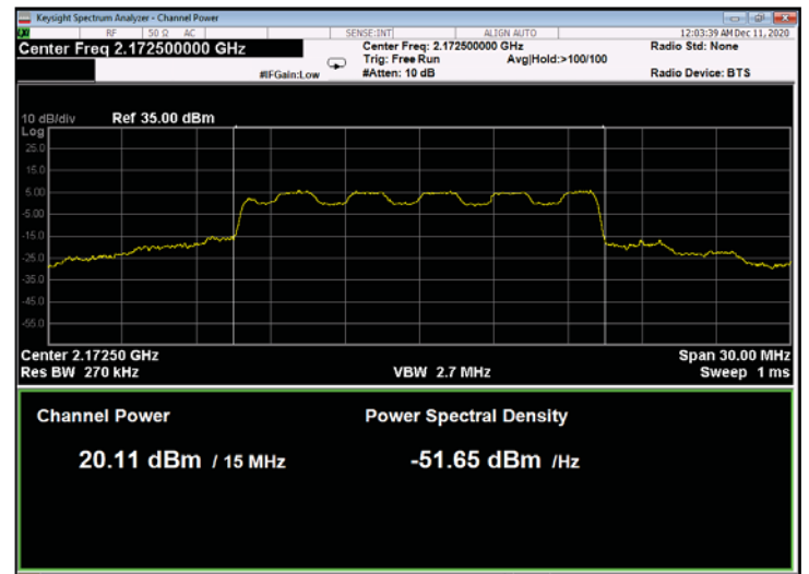
Figure 30: 16QAM 15MHz B.W.; 2172.5MHz, 15kHz
