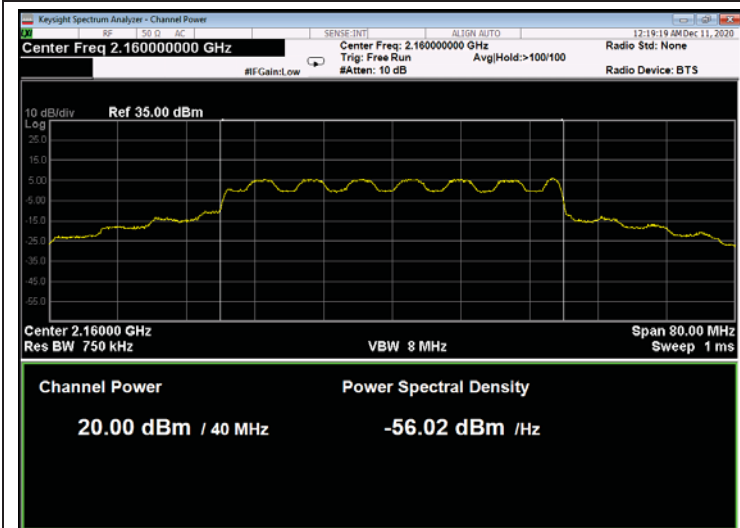
Figure 57: 16QAM 40MHz B.W.; 2160.0MHz, 15kHz
