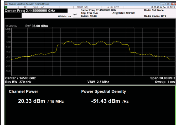
Figure 29: 16QAM 15MHz B.W.; 2145.0MHz, 60kHz
