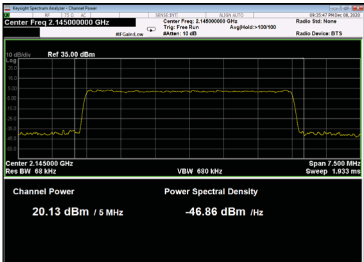
Figure 77: 64QAM 5MHz B.W.; 2145MHz, 15kHz
