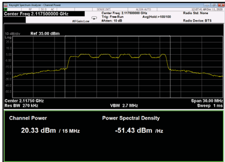
Figure 25: 16QAM 15MHz B.W.; 2117.5MHz, 30kHz
