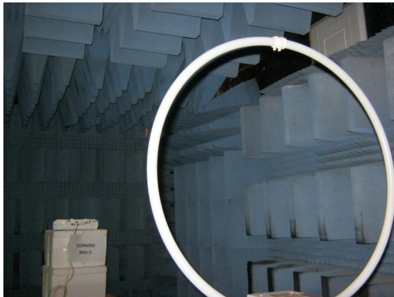
Radiated Emission Test 0.009MHz-30MHz
