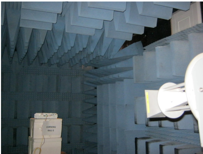
Radiated Emission Test 18-20.0GHz
