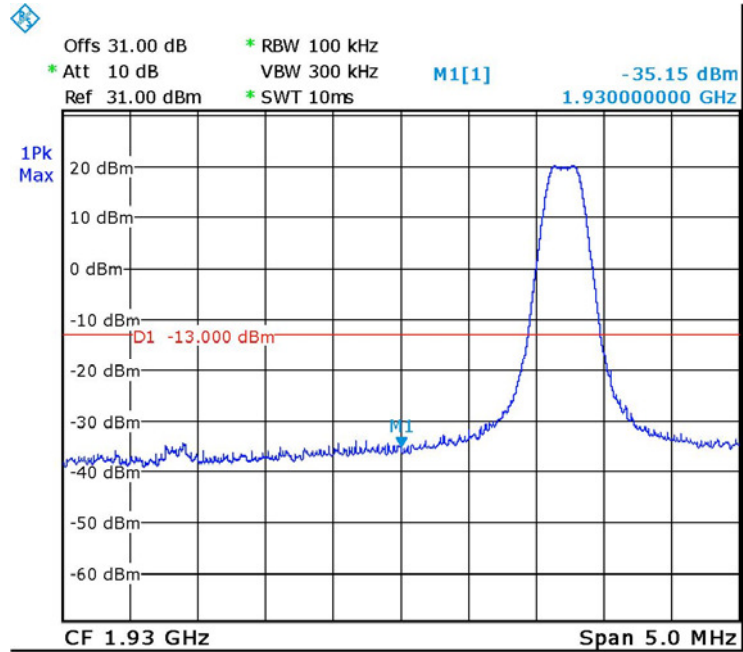
Figure 54. — GSM - 1931.2 MHz
