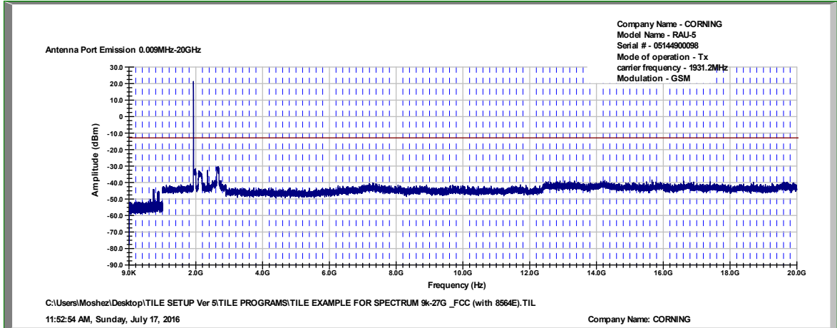
Figure 44. — GSM - 1931.2 MHz
