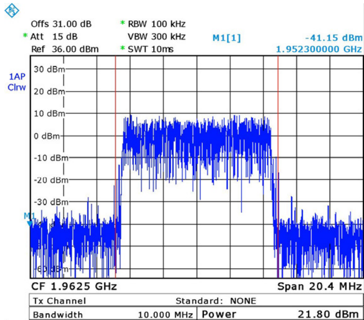
Figure 12. — LTE 64QAM 1962.5 MHz
