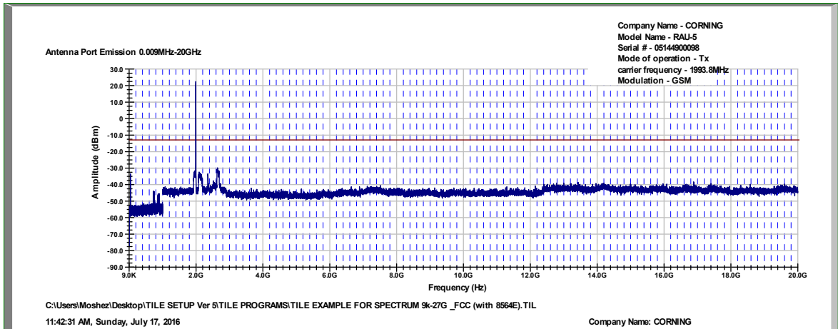
Figure 46. — GSM - 1993.8 MHz
