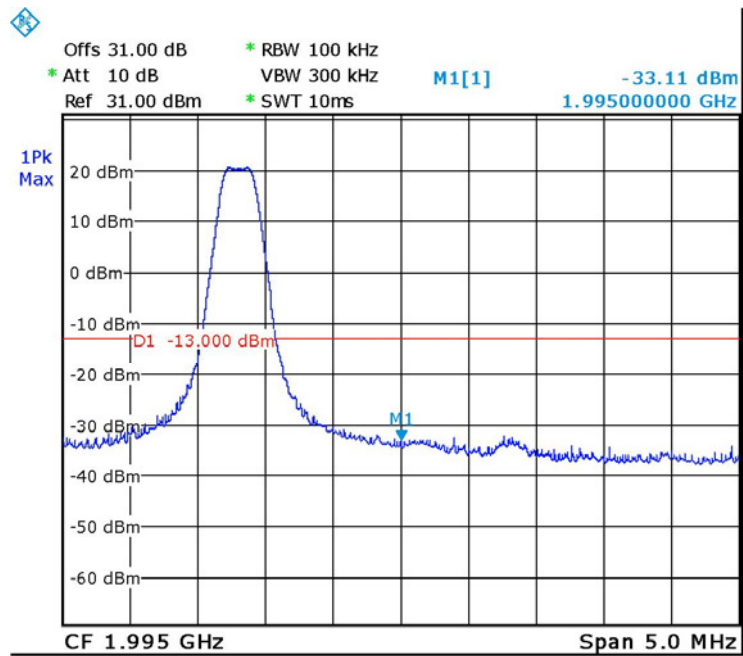
Figure 55. — GSM - 1993.8 MHz
