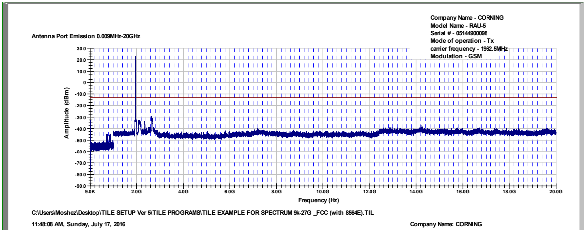
Figure 45. — GSM - 1962.5 MHz
