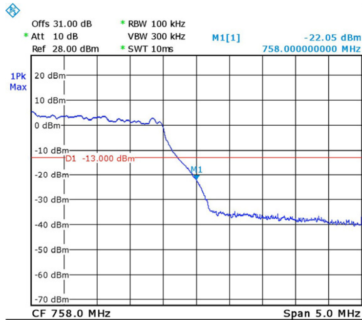
Figure 53. — 64QAM 753.0 MHz
