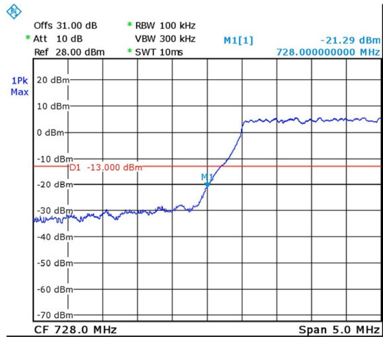
Figure 52.—64QAM 733.0 MHz
