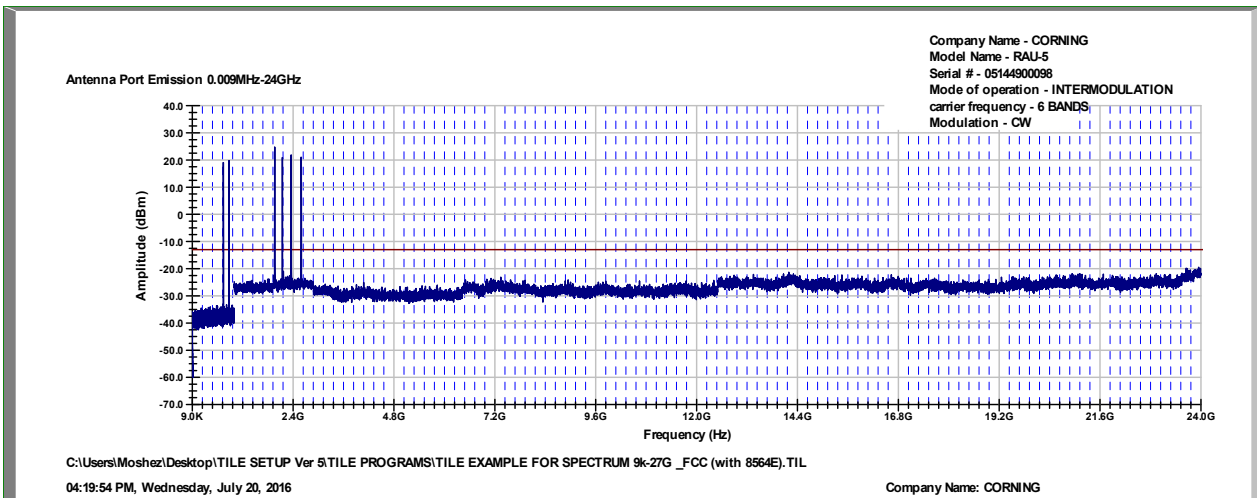
Figure 61 Intermodulation Conducted
