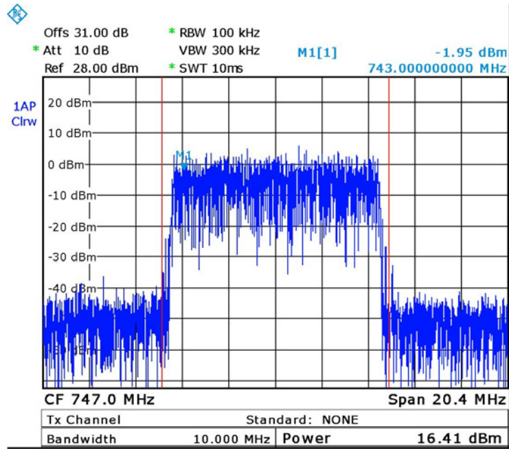
Figure 15. — 16QAM 747 MHz
