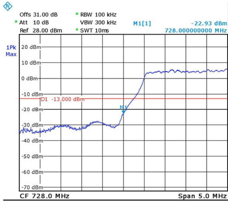
Figure 56. — QPSK 733.0 MHz
