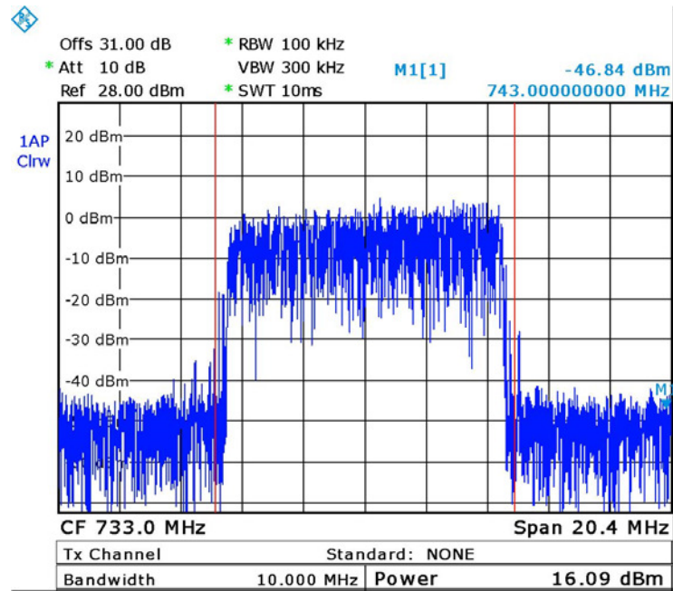
Figure 11. — 64QAM, 733 MHz
