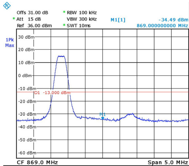
Figure 94. — GSM - 867.8 MHz
