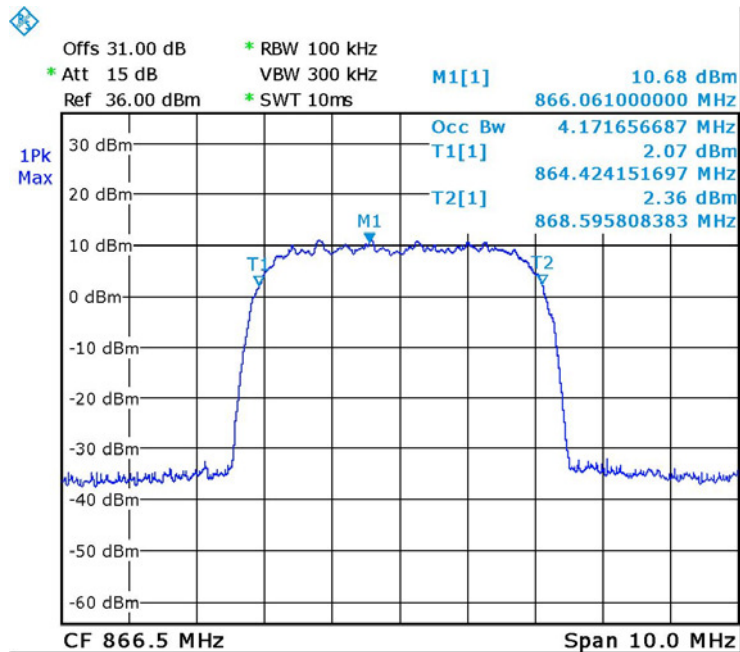
Figure 76. — 866.5MHz WCDMA Input
