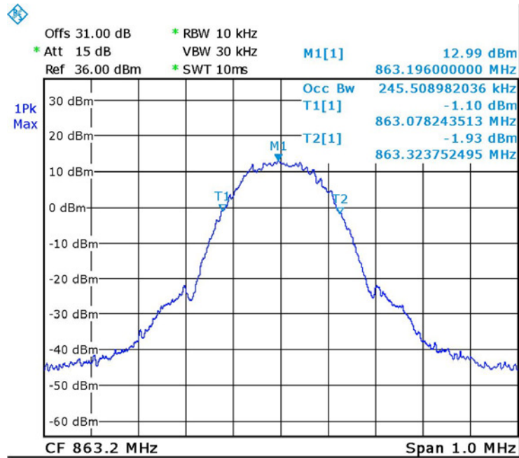
Figure 78. — 863.2MHz GSM Input
