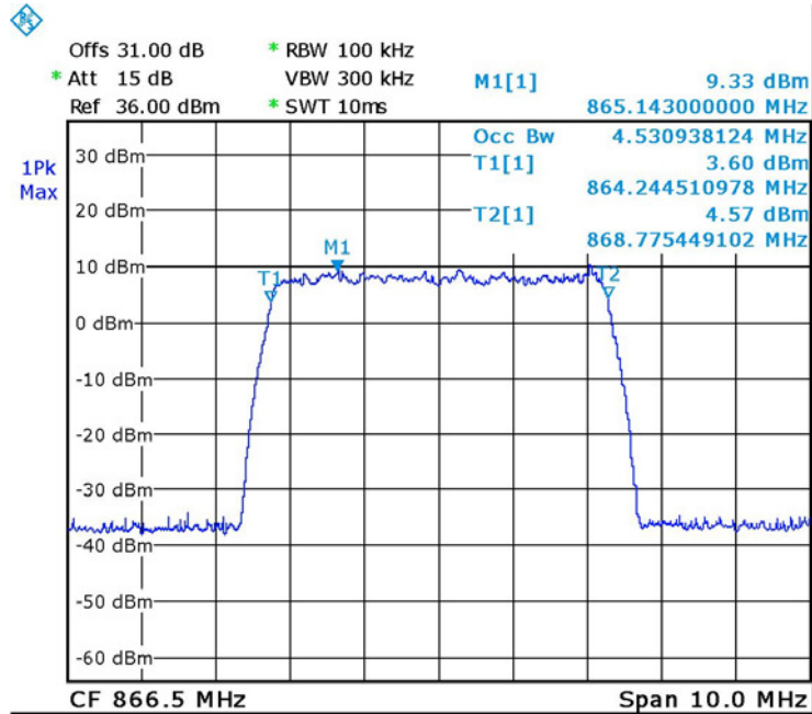
Figure 72. — 866.5MHz LTE 64QAM Input
