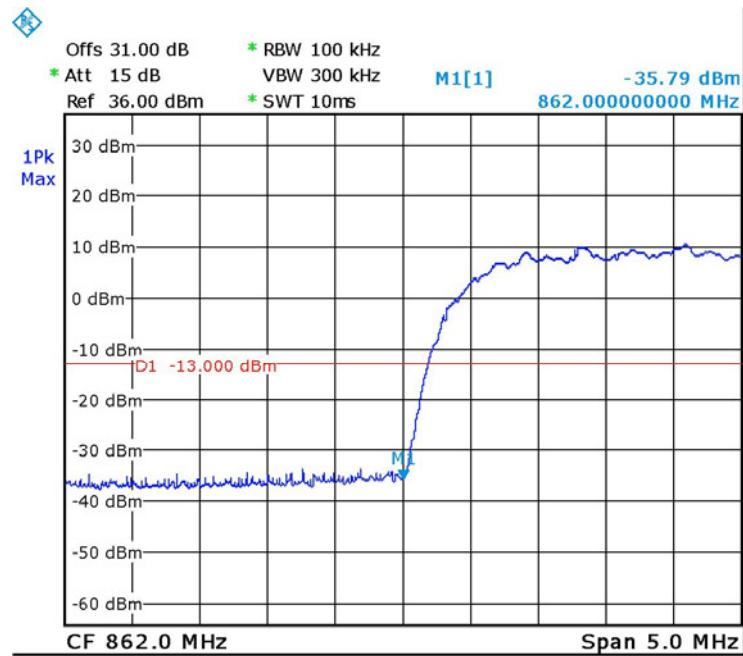
Figure 95. — W-CDMA - 864.5 MHz
