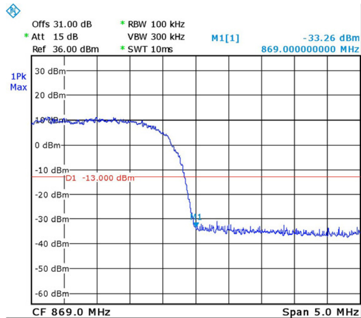
Figure 96. — W-CDMA - 866.5 MHz
