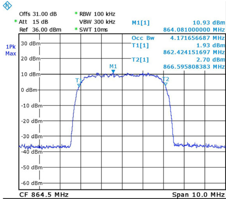
Figure 74. — 864.5MHz WCDMA Input
