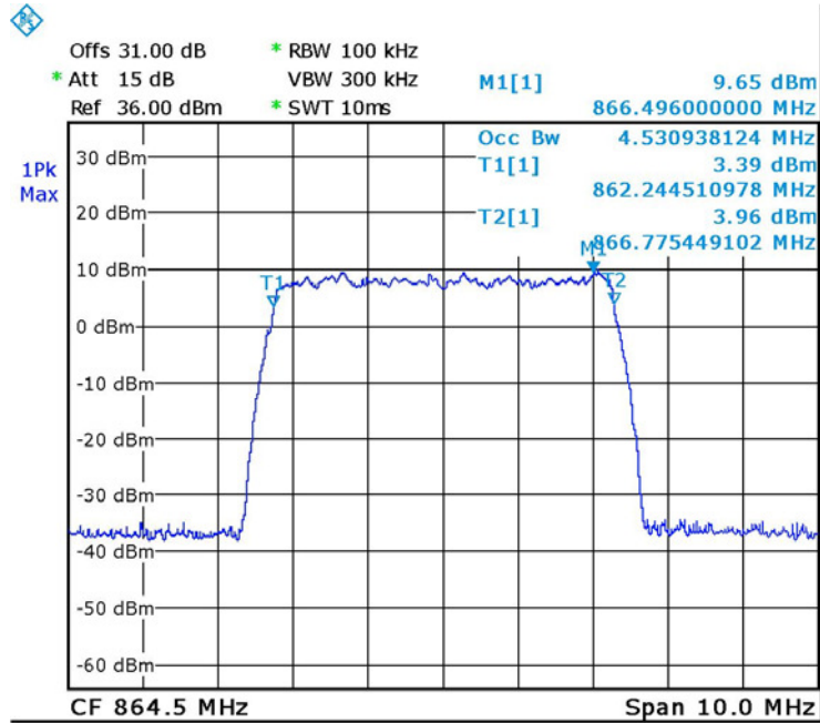
Figure 70. — 864.5MHz LTE 64QAM Input
