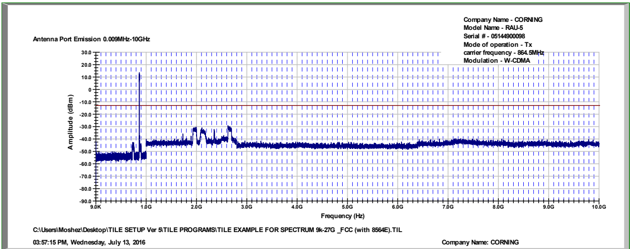
Figure 87. — 864.5 WCDMA
