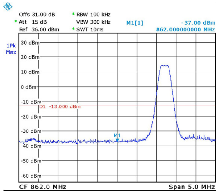
Figure 93. — GSM - 863.2MHz
