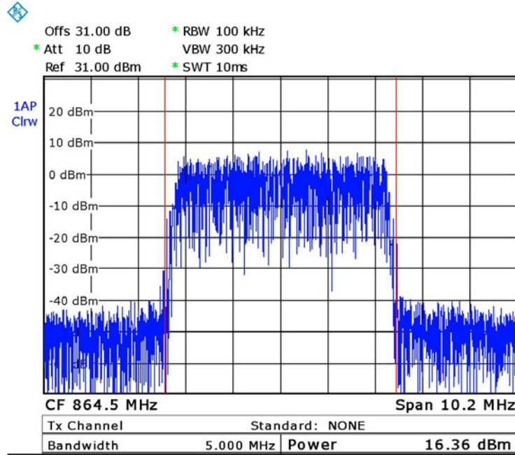
Figure 62. — 864.5 MHz – LTE 64QAM
