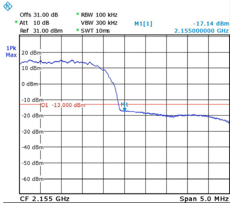
Figure 57. — W-CDMA 2152.5 MHz
