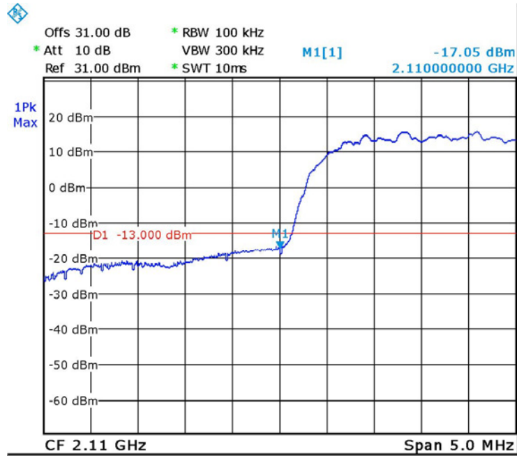
Figure 56. — W-CDMA 2112.5 MHz
