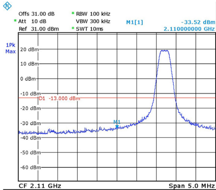
Figure 52. — GSM 2111.2 MHz
