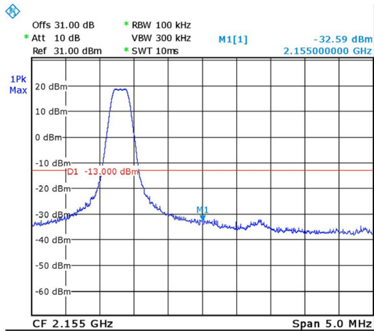
Figure 53. — GSM 2153.8 MHz
