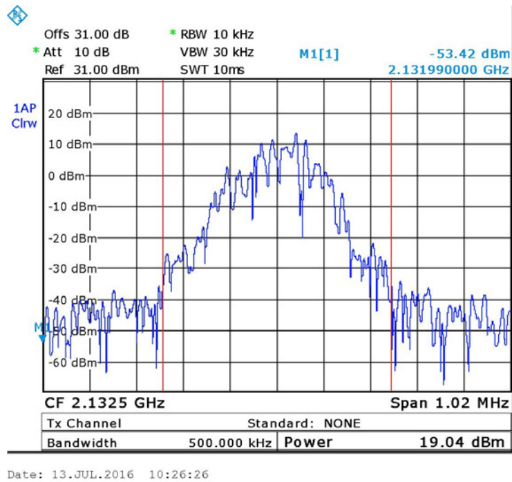
Figure 12. — GSM (2132.5.0MHz)
