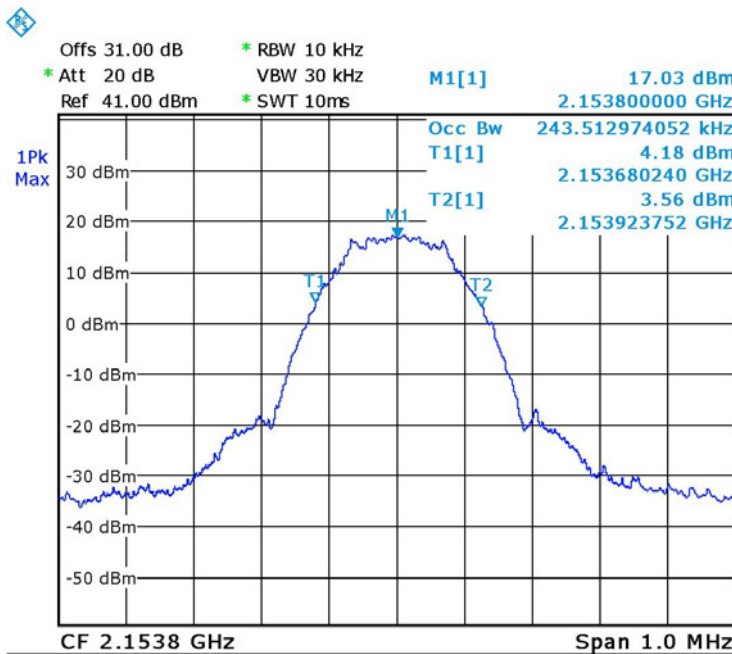
Figure 33. — GSM (2153.8 MHz) OUT
