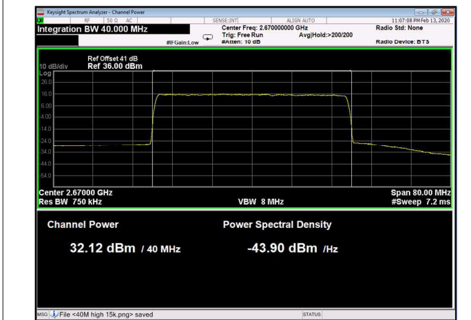
Figure 96: 64QAM 40MHz B.W.; 2670.0MHz, 30kHz
