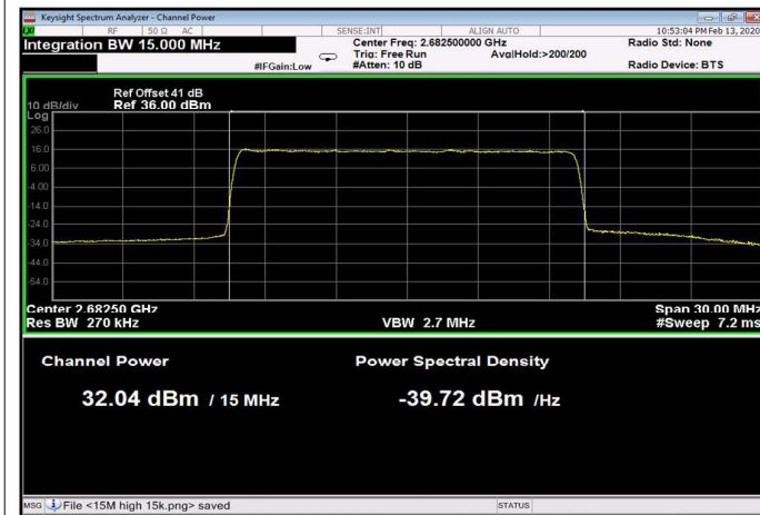
Figure 78: 64QAM 15MHz; 2682.5MHz B.W., 30kHz
