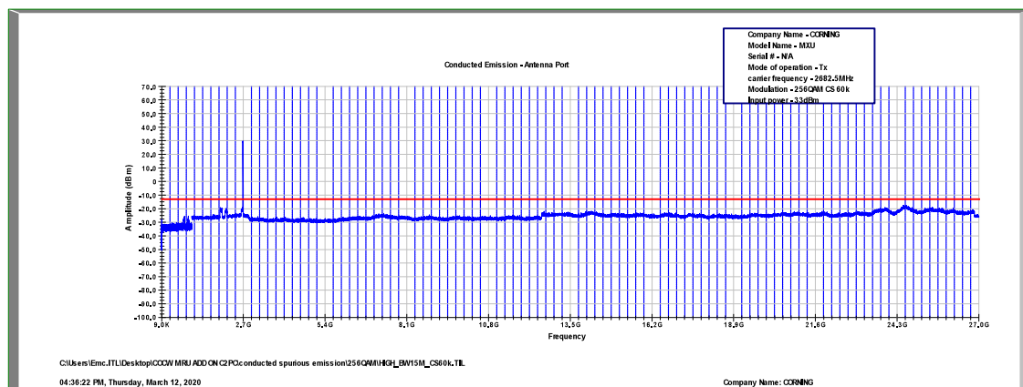
Figure 559: Spurious Emissions at Antenna Terminal 256QAM, 2682.5MHz, B.W. 15MHz, Sub Carrier 60kHz
