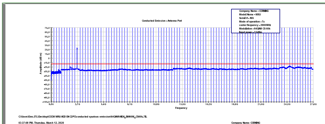
Figure 535: Spurious Emissions at Antenna Terminal 64QAM, 2660.0MHz, B.W. 60MHz, Sub Carrier 30kHz
