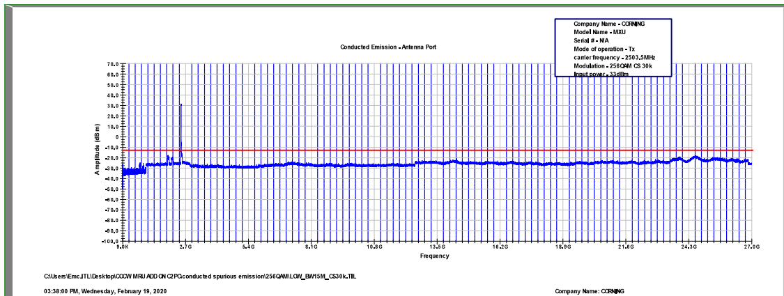
Figure 554: Spurious Emissions at Antenna Terminal 256QAM, 2503.5MHz, B.W. 15MHz, Sub Carrier 30kHz
