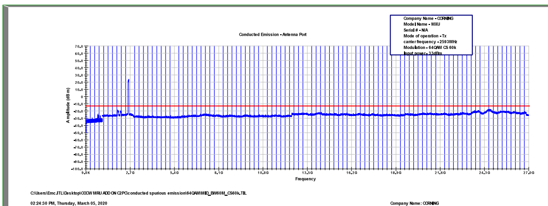
Figure 534: Spurious Emissions at Antenna Terminal 64QAM, 2593.0MHz, B.W. 60MHz, Sub Carrier 60kHz
