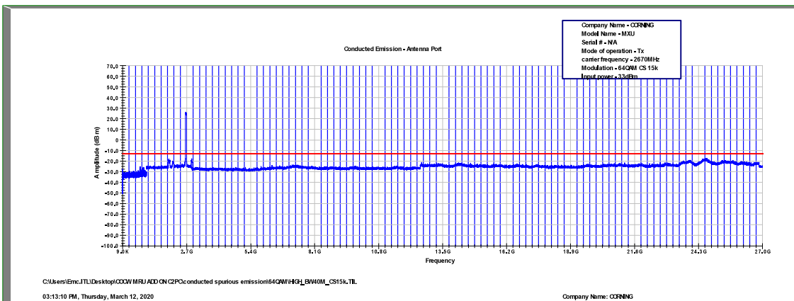
Figure 523: Spurious Emissions at Antenna Terminal 64QAM, 2670.0MHz, B.W. 40MHz, Sub Carrier 15kHz
