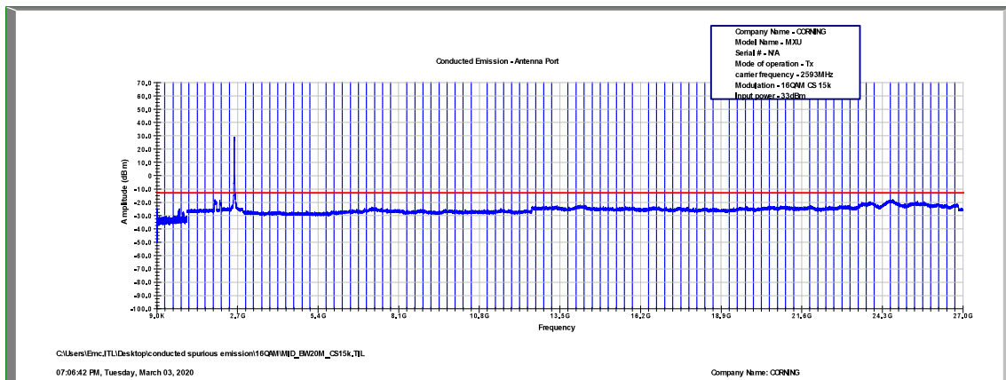
Figure 465: Spurious Emissions at Antenna Terminal 16QAM, 2593.0MHz, B.W. 20MHz, Sub Carrier 15kHz
