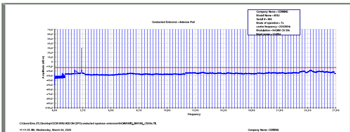
Figure 498: Spurious Emissions at Antenna Terminal 64QAM, 2593.0MHz, B.W. 10MHz, Sub Carrier 30kHz
