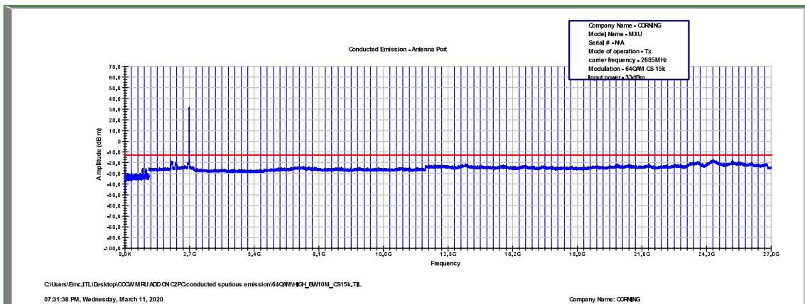
Figure 496: Spurious Emissions at Antenna Terminal 64QAM, 2685.0MHz, B.W. 10MHz, Sub Carrier 15kHz
