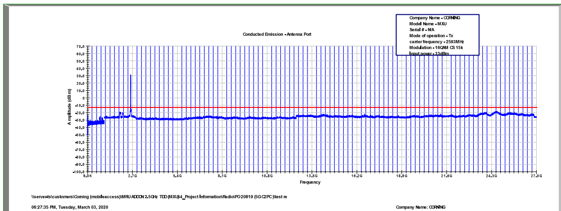
Figure 447: Spurious Emissions at Antenna Terminal 16QAM, 2593.0MHz, B.W. 10MHz, Sub Carrier 15kHz
