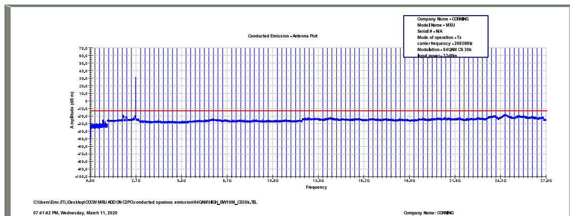
Figure 499: Spurious Emissions at Antenna Terminal 64QAM, 2685.0MHz, B.W. 10MHz, Sub Carrier 30kHz
