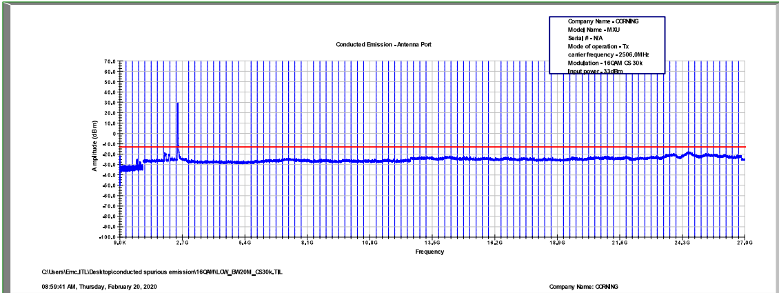
Figure 467: Spurious Emissions at Antenna Terminal 16QAM, 2506.0MHz, B.W. 20MHz, Sub Carrier 30kHz
