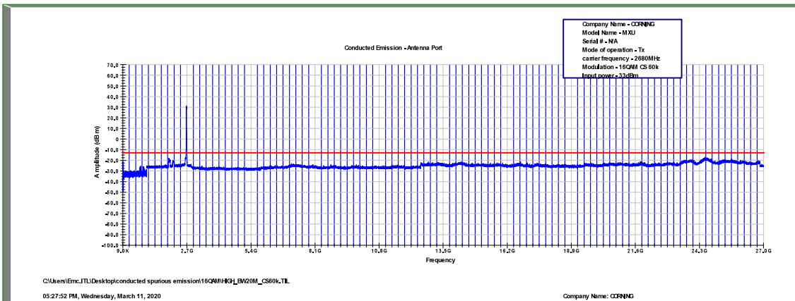
Figure 472: Spurious Emissions at Antenna Terminal 16QAM, 2680.0MHz, B.W. 20MHz, Sub Carrier 60kHz
