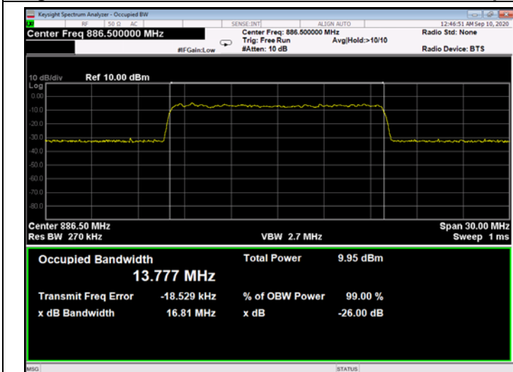
Figure 324: QPSK 15MHz B.W.; 886.5MHz, 30kHz - Input
