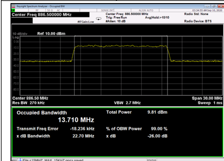
Figure 282: 256QAM 15MHz B.W.; 886.5MHz, 30kHz - Input
