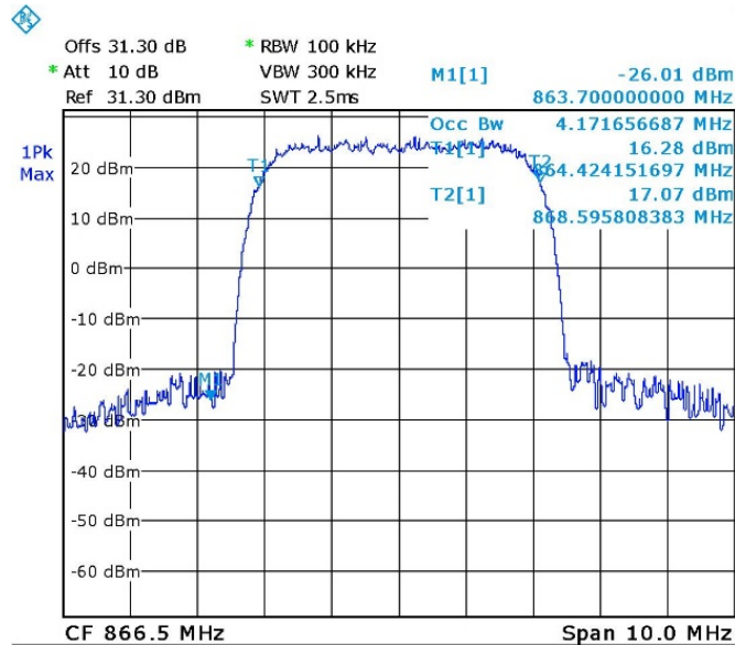
Figure 73. — 866.5MHz WCDMA Input
