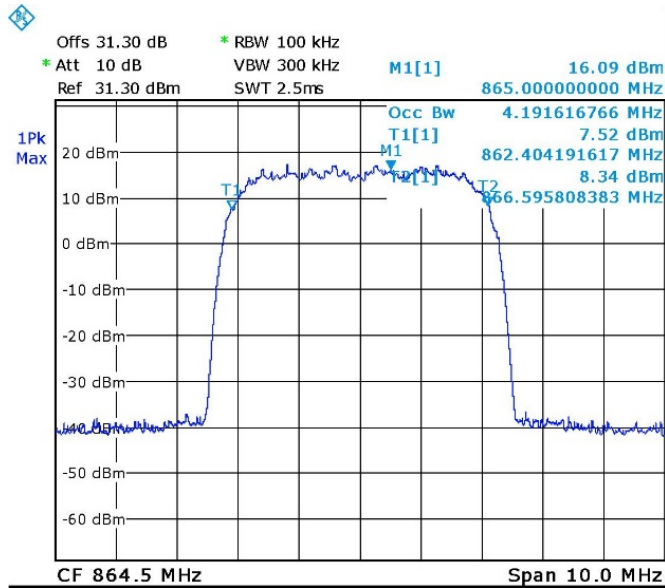
Figure 71. — 864.5MHz WCDMA Input
