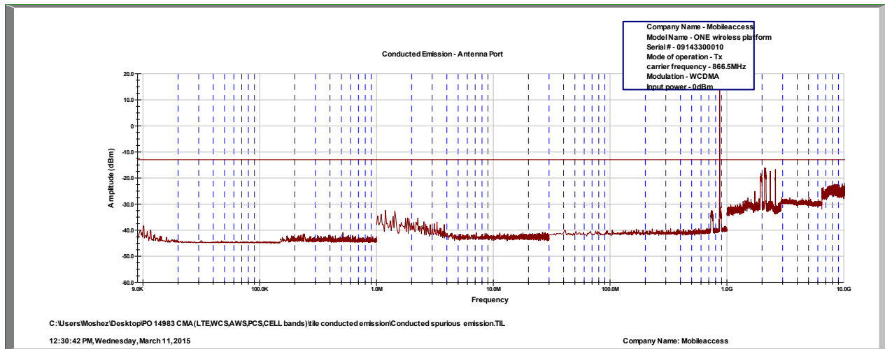
Figure 85. — 866.5 WCDMA
