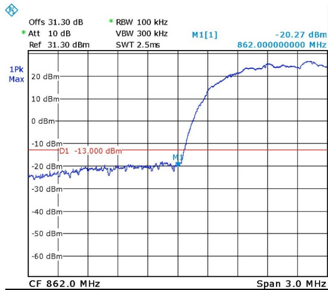
Figure 92. — W-CDMA - 864.5 MHz
