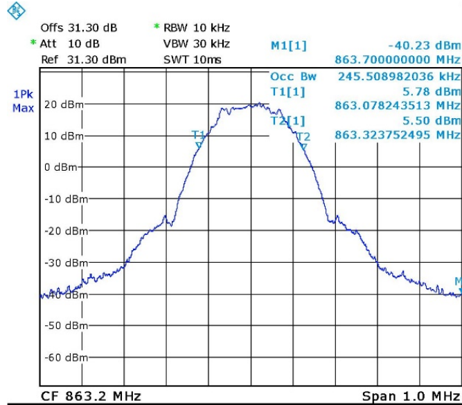
Figure 75. — 863.2MHz GSM Input
