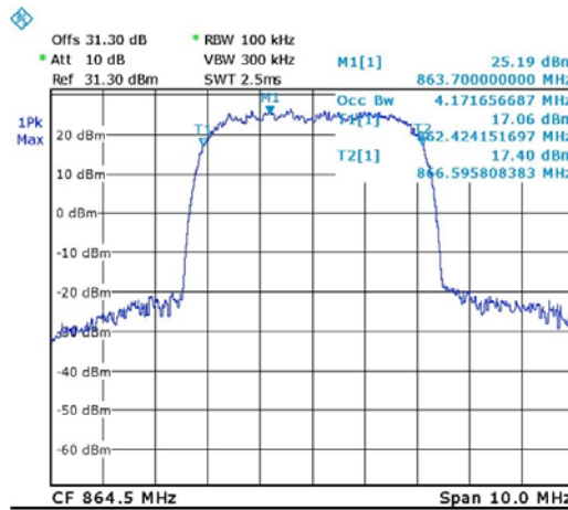
Figure 71. — 864.5MHz WCDMA Input
