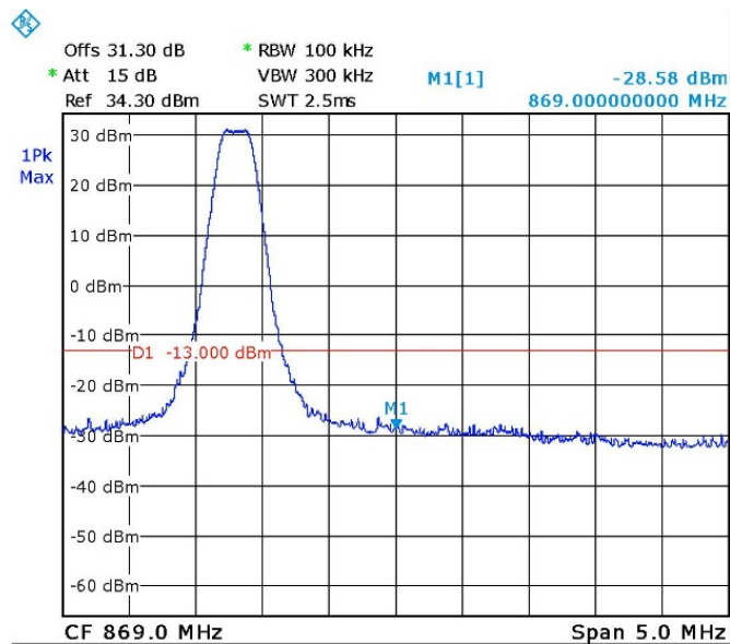
Figure 91. — GSM - 867.8 MHz
