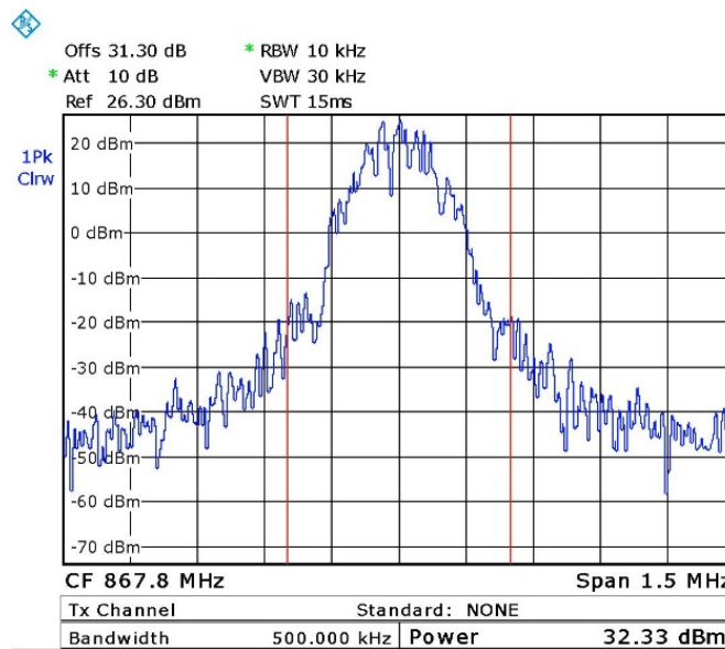
Figure 62. — 867.8 MHz – GSM
