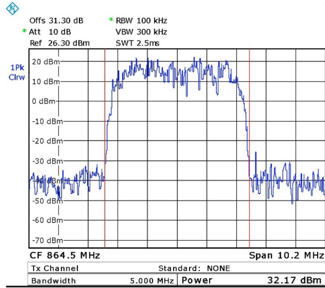
Figure 63.—864.5 MHz – WCDMA
