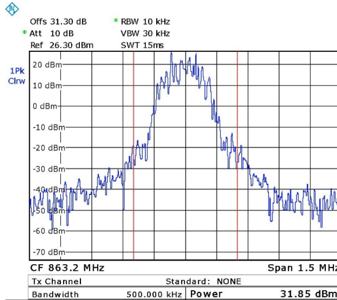
Figure 61. — 863.2 MHz – GSM
