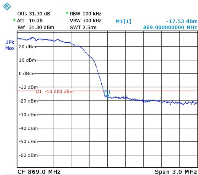
Figure 93. — W-CDMA - 866.5 MHz
