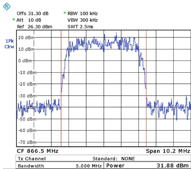
Figure 64. — 866.5 MHz – WCDMA
