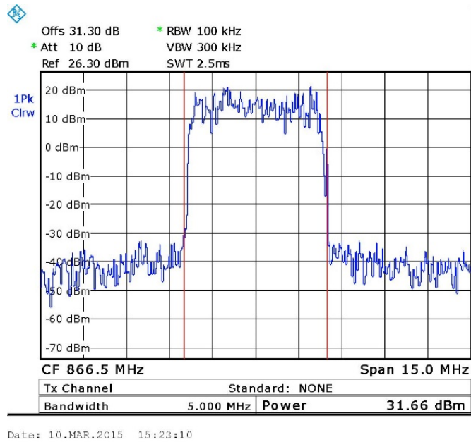
Figure 60. — 866.5 MHz – LTE 64QAM
