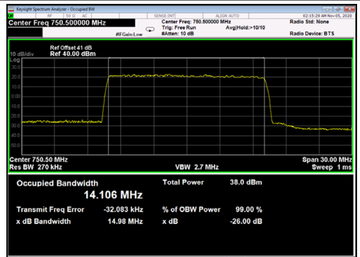
Figure 359: 256QAM 15MHz B.W.; 750.5MHz, 15kHz - Output
