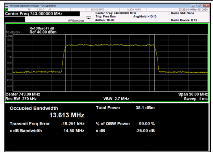
Figure 357: 256QAM 15MHz B.W.; 743.0MHz, 30kHz - Output
