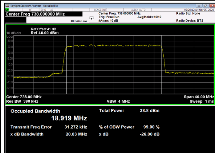
Figure 362: 256QAM 20MHz B.W.; 738.0MHz, 15kHz - Output
