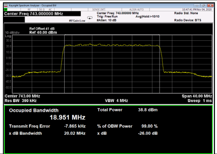
Figure 332: 64QAM 20MHz B.W.; 743.0MHz, 15kHz - Output
