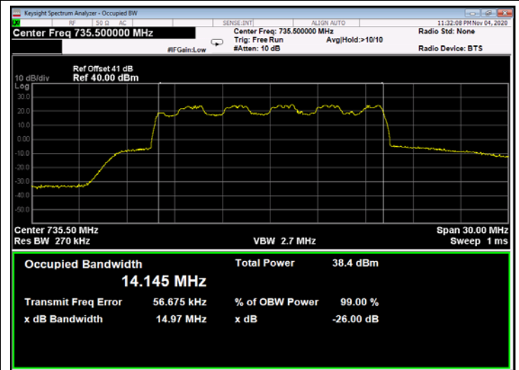
Figure 287: 16QAM 15MHz B.W.; 735.5MHz, 15kHz - Output
