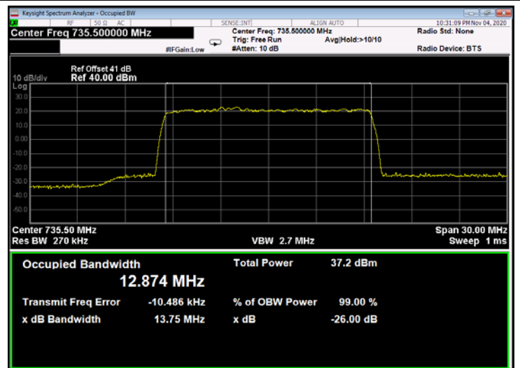
Figure 322: 64QAM 15MHz B.W.; 735.5MHz, 60kHz - Output
