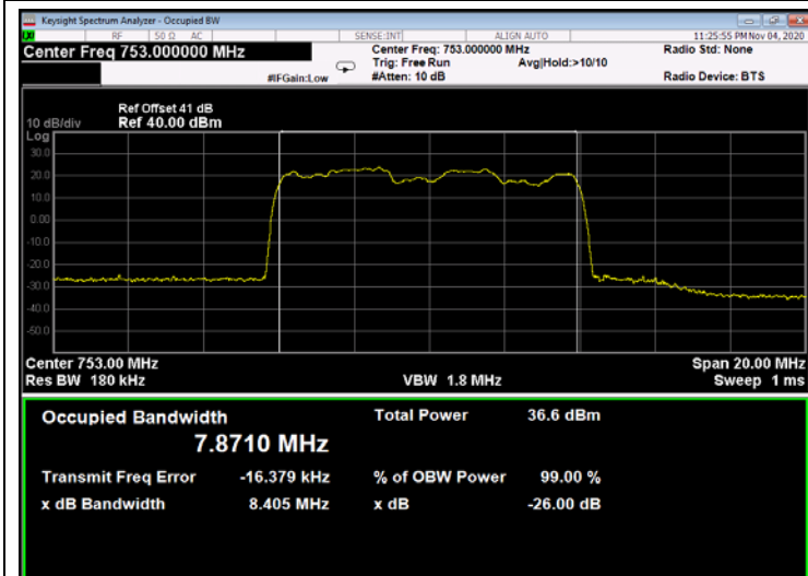
Figure 286: 16QAM 10MHz B.W.; 753.0MHz, 60kHz - Output
