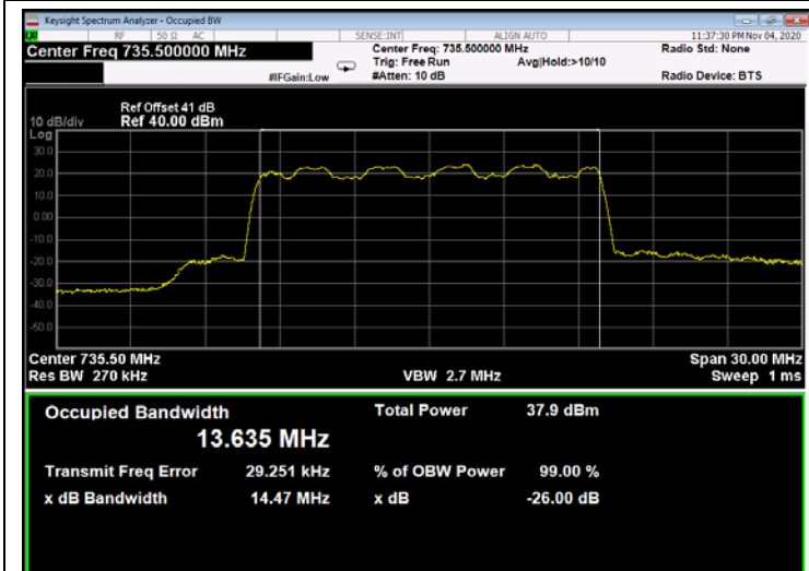
Figure 288: 16QAM 15MHz B.W.; 735.5MHz, 30kHz - Output
