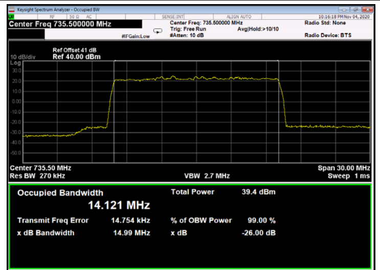
Figure 320: 64QAM 15MHz B.W.; 735.5MHz, 15kHz- Output
