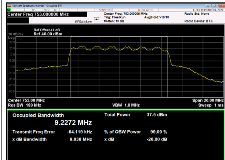
Figure 284: 16QAM 10MHz B.W.; 753.0MHz, 15kHz - Output
