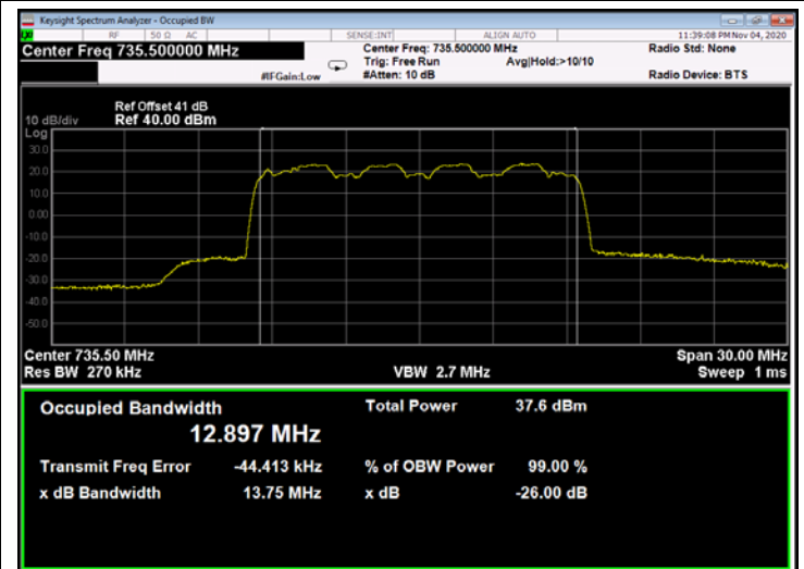
Figure 289: 16QAM 15MHz B.W.; 735.5MHz, 60kHz - Output
