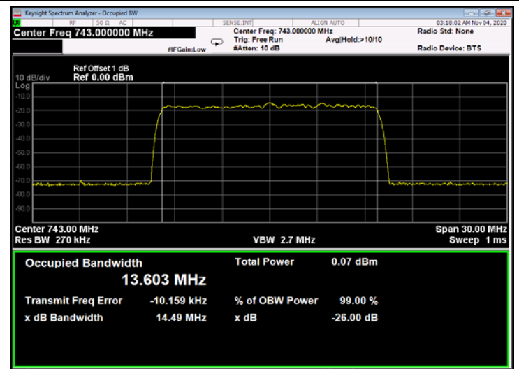
Figure 192: 64QAM 15MHz B.W.; 743.0MHz, 30kHz - Input
