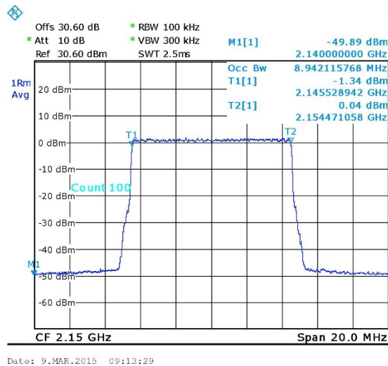
Figure 23. — LTE 64QAM (2150.0 MHz) IN
