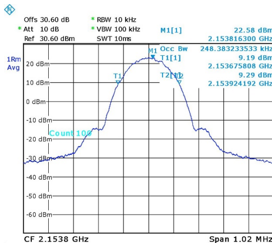
Figure 30. — GSM (2153.8 MHz) OUT
