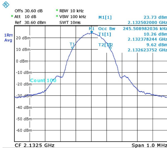
Figure 28. — GSM (2132.5 MHz) OUT
