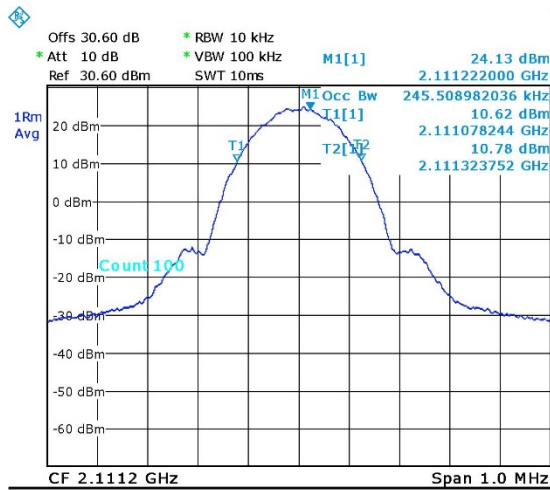
Figure 25. — GSM (2111.2 MHz) IN
