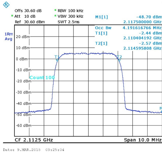
Figure 31. — W-CDMA (2112.5 MHz) IN
