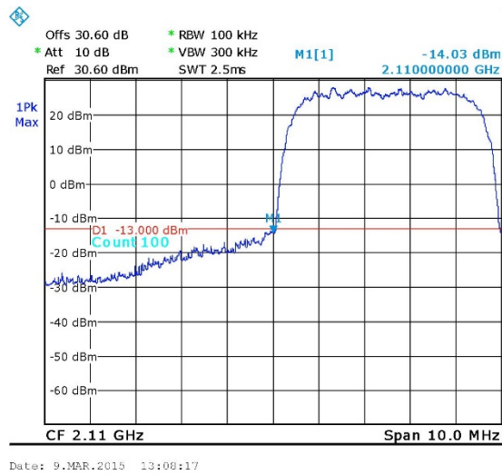
Figure 53. — W-CDMA 2112.50 MHz
