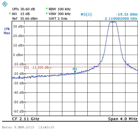
Figure 49. — GSM 2111.20 MHz
