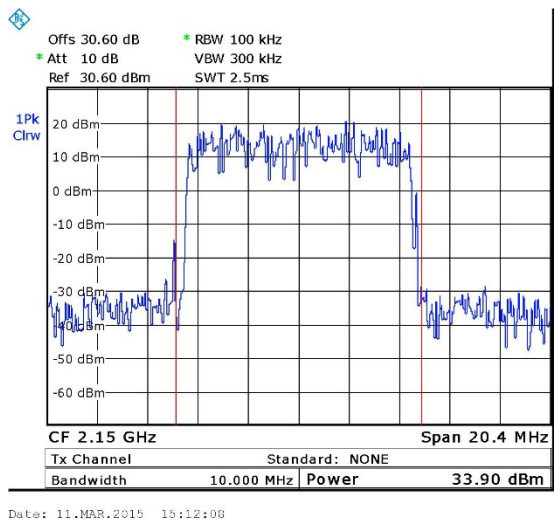
Figure 13. — LTE 64QAM (2150.0MHz)
