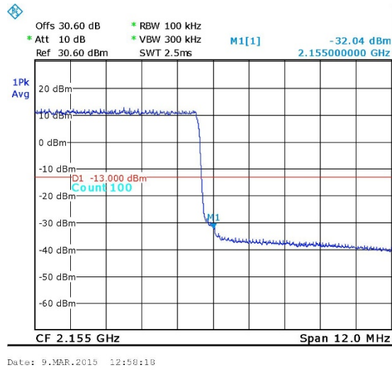
Figure 52. — LTE 64QAM 2150.00 MHz
