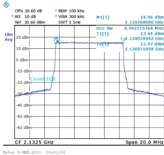
Figure 22. — LTE 64QAM (2132.5 MHz) OUT
