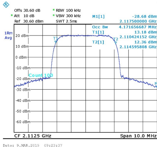
Figure 32. — W-CDMA (2112.5 MHz) OUT
