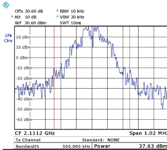
Figure 8. — GSM (2111.2 MHz)
