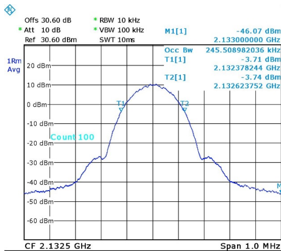
Figure 27. — GSM (2132.5 MHz) IN
