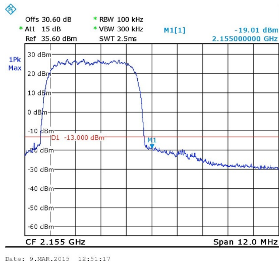
Figure 54. — W-CDMA 2152.50 MHz
