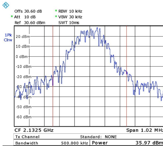
Figure 9. — GSM (2132.5 MHz)
