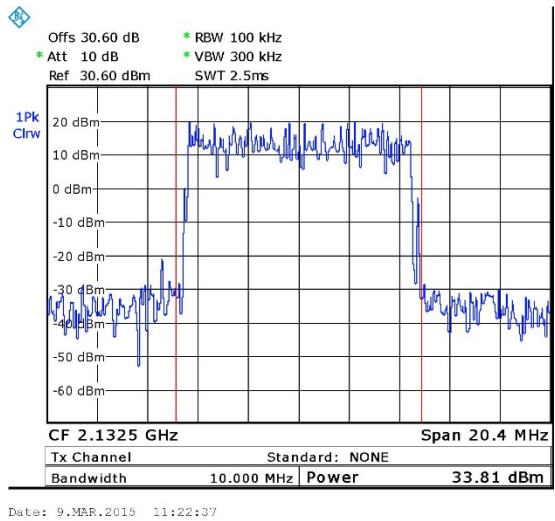
Figure 12. — LTE 64QAM (2132.5 MHz)
