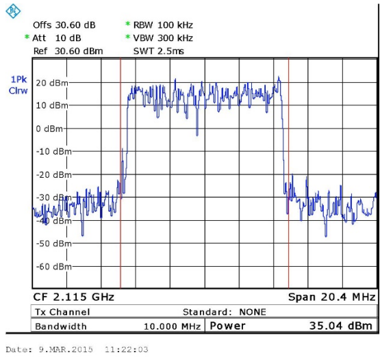
Figure 11. — LTE 64QAM (2115.0 MHz)
