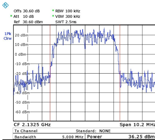
Figure 15. — W-CDMA (2132.5 MHz)
