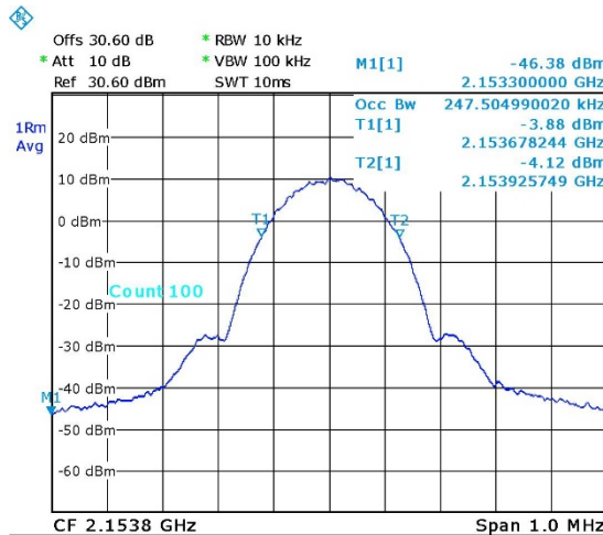
Figure 29. — GSM (2153.8 MHz) IN
