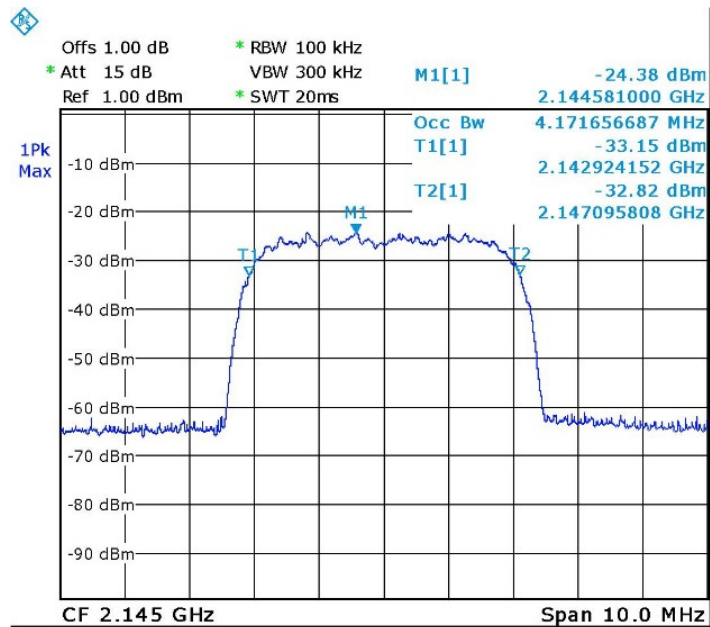
Figure 35. — W-CDMA (2145.0MHz) IN
