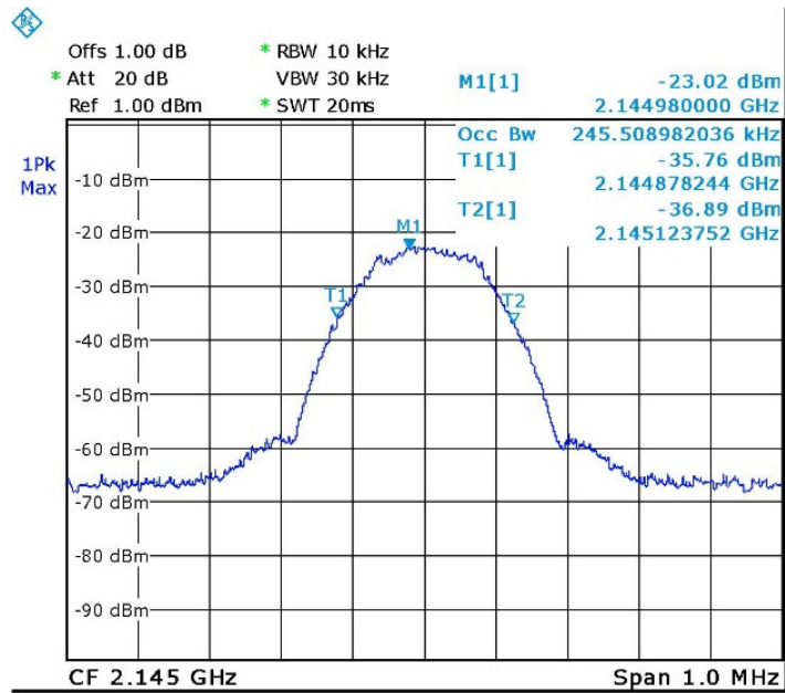
Figure 29. — GSM (2145.0MHz) IN
