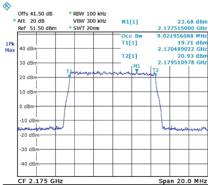
Figure 25. — LTE 64QAM (2175.0 MHz) IN
