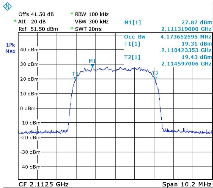
Figure 34. — W-CDMA (2112.5 MHz) OUT
