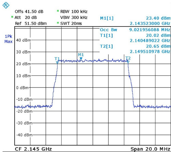
Figure 23. — LTE 64QAM (2145.0MHz) IN
