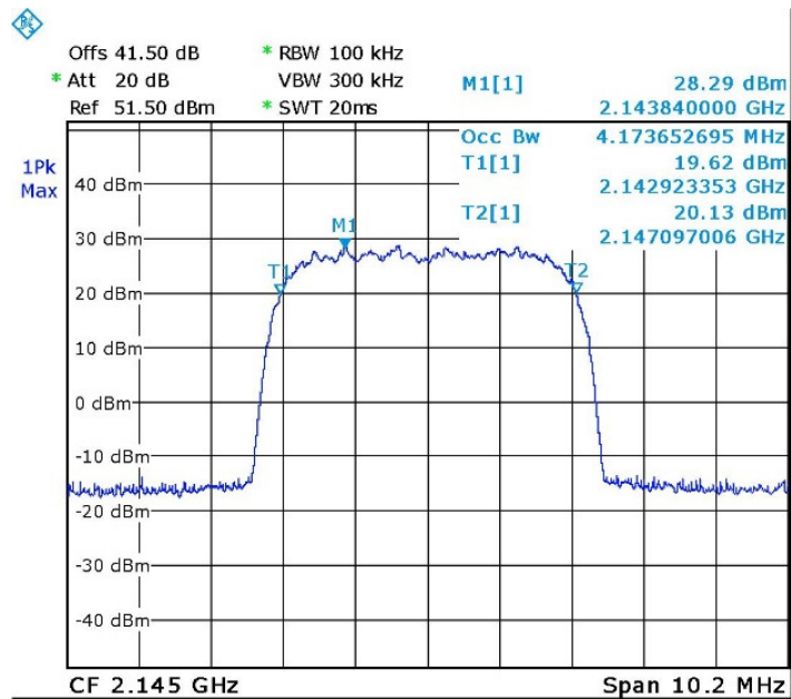
Figure 36. — W-CDMA (2145.0MHz) OUT
