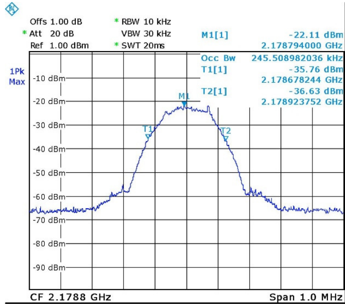
Figure 31. — GSM (2178.8 MHz) IN
