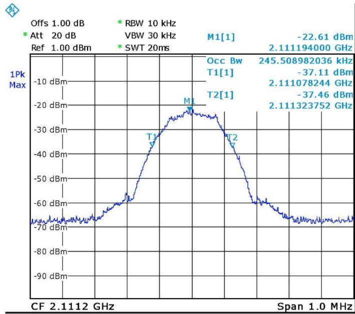
Figure 27. — GSM (2111.2 MHz) IN
