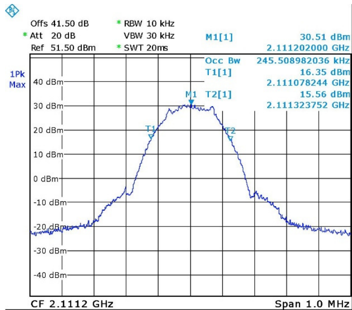
Figure 28. — GSM (2111.2 MHz) OUT
