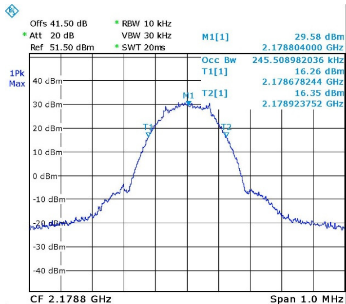
Figure 32. — GSM (2178.8 MHz) OUT
