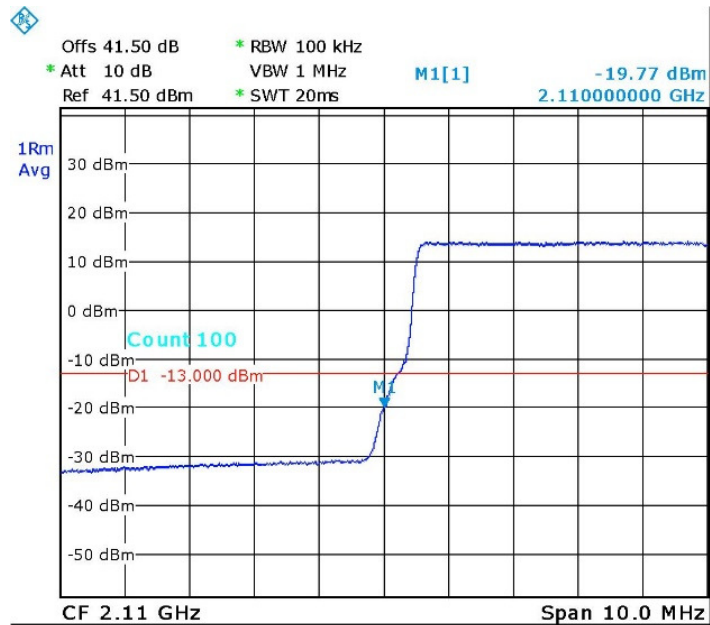
Figure 53. — LTE 64QAM 2115.0 MHz
