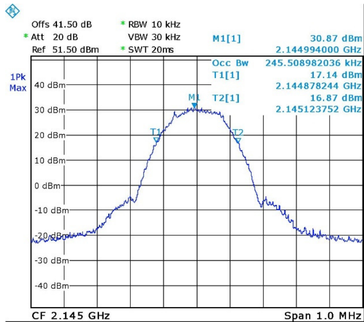
Figure 30. — GSM (2145.0MHz) OUT
