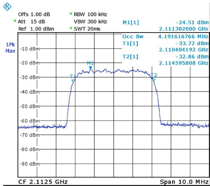
Figure 33. — W-CDMA (2112.5 MHz) IN
