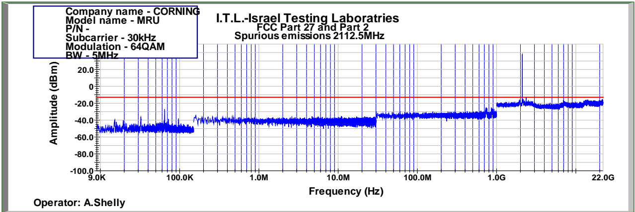
Figure 870: Spurious Emissions at Antenna Terminal 64QAM 5MHz B.W.; 2112.5MHz, 30kHz
