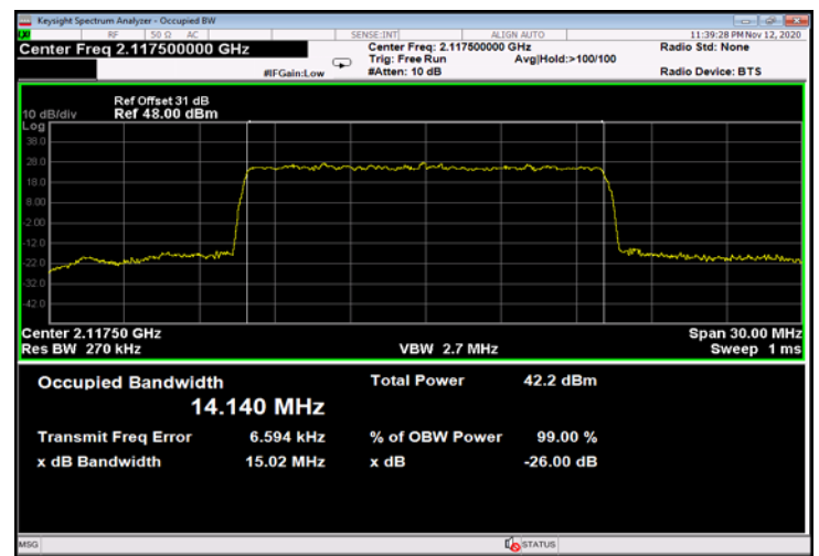
Figure 750: QPSK 15MHz B.W.; 2117.5MHz, 15kHz - Output
