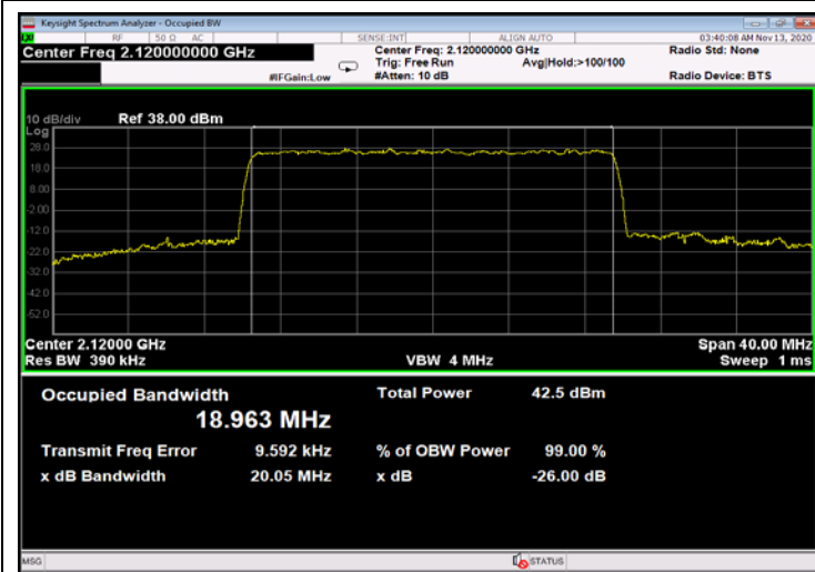
Figure 693: 256QAM 20MHz B.W.; 2120.0MHz, 15kHz - Output
