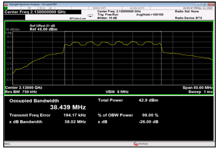
Figure 580: 16QAM 40MHz B.W.; 2130.0MHz, 30kHz - Output
