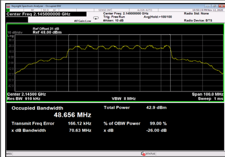
Figure 591: 16QAM 50MHz B.W.; 2145.0MHz, 15kHz - Output
