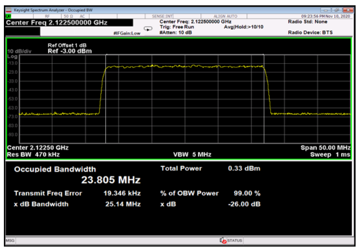
Figure 504: QPSK 25MHz B.W.; 2122.5MHz, 15kHz - Input
