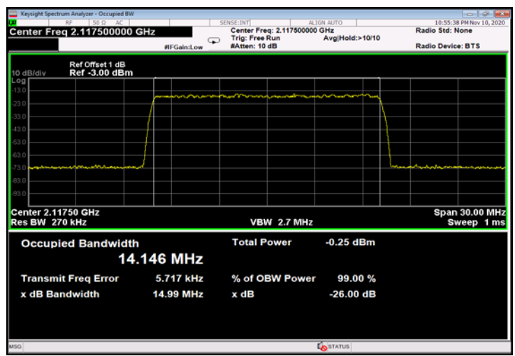
Figure 420: 256QAM 15MHz B.W.; 2117.5MHz, 15kHz - Input
