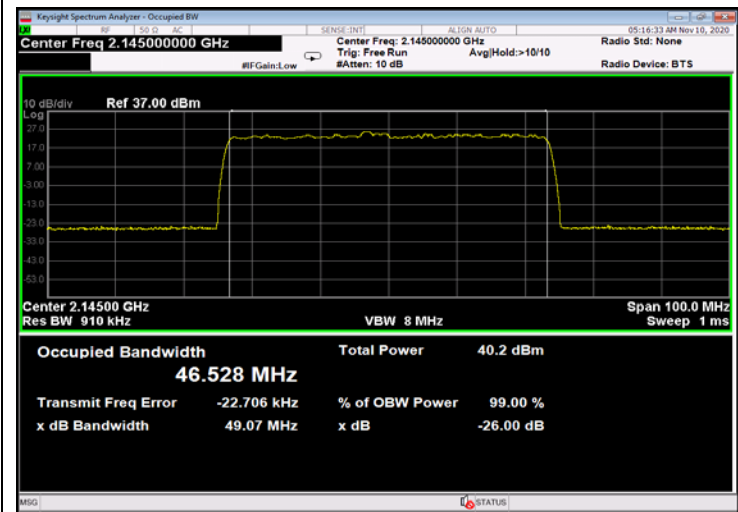
Figure 395: 64QAM 50MHz B.W.; 2145.0MHz, 60kHz - Input
