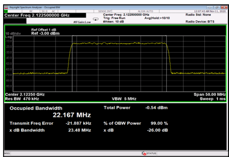
Figure 440: 256QAM 25MHz B.W.; 2122.5MHz, 60kHz - Input
