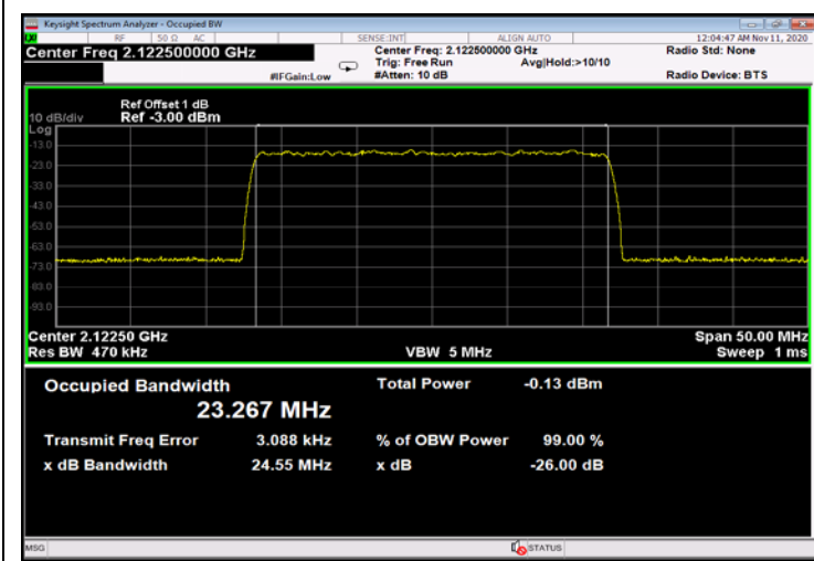
Figure 439: 256QAM 25MHz B.W.; 2122.5MHz, 30kHz - Input
