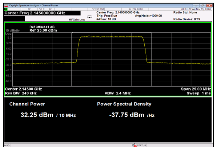
Figure 86: 64QAM 10MHz B.W.; 2145MHz, 60kHz
