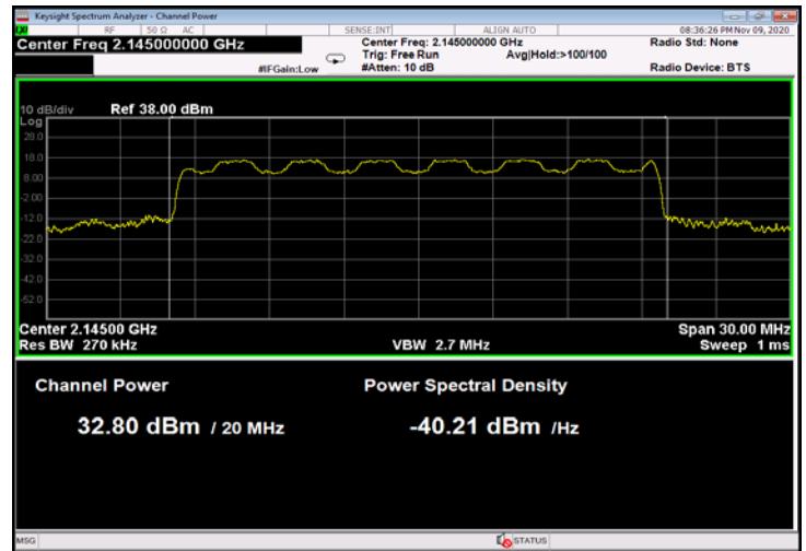
Figure 36: 16QAM 20MHz B.W.; 2145.0MHz, 15kHz
