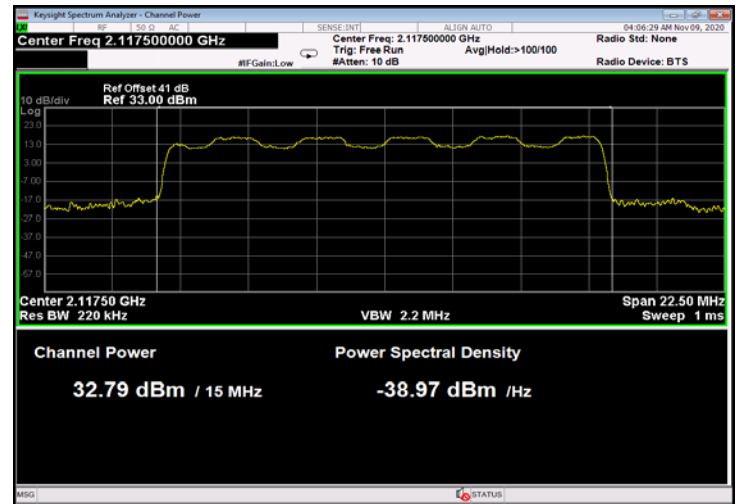
Figure 24: 16QAM 15MHz B.W.; 2117.5MHz, 15kHz
