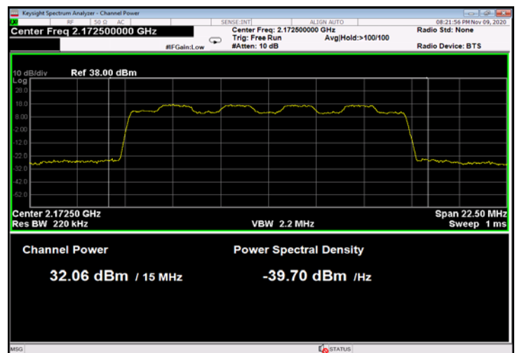
Figure 32: 16QAM 15MHz B.W.; 2172.5MHz, 60kHz
