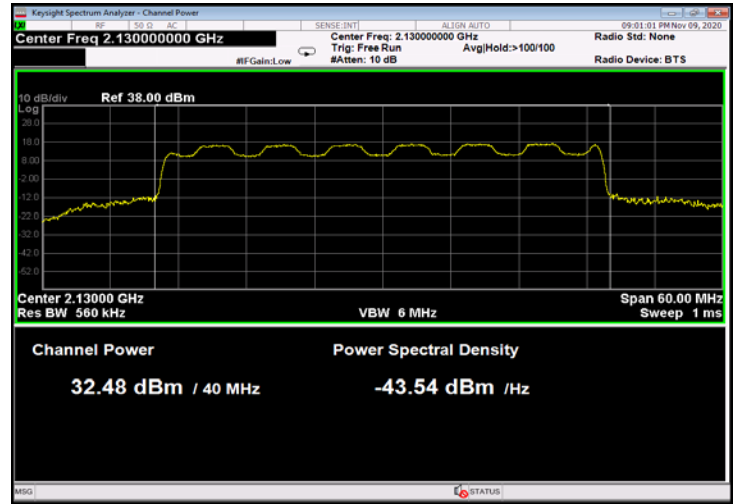
Figure 52: 16QAM 40MHz B.W.; 2130.0MHz, 30kHz
