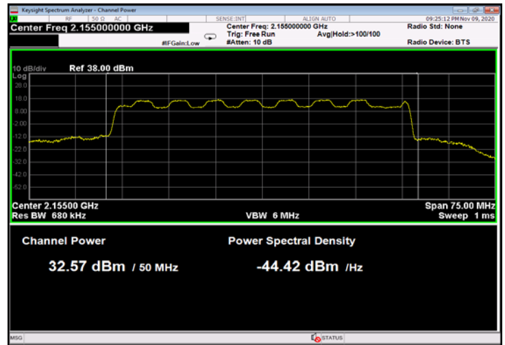
Figure 68: 16QAM 50MHz B.W.; 2155.0MHz, 60kHz
