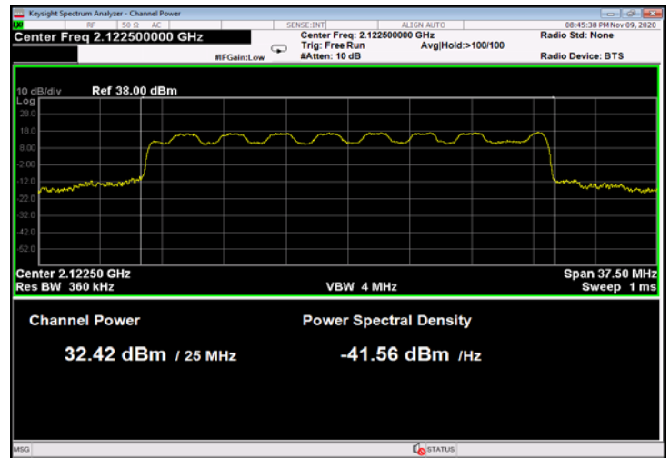
Figure 42: 16QAM 25MHz B.W.; 2122.5MHz, 15kHz
