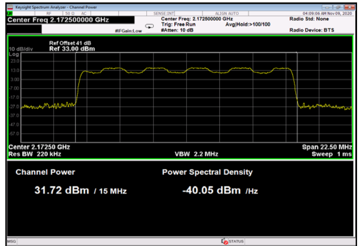
Figure 30: 16QAM 15MHz B.W.; 2172.5MHz, 15kHz
