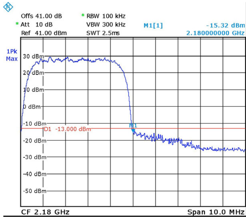
Figure 55. — W-CDMA 2177.5 MHz
