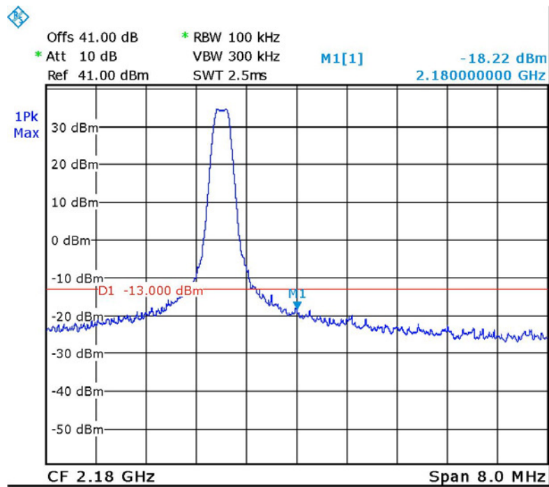
Figure 51. — GSM 2178.8 MHz
