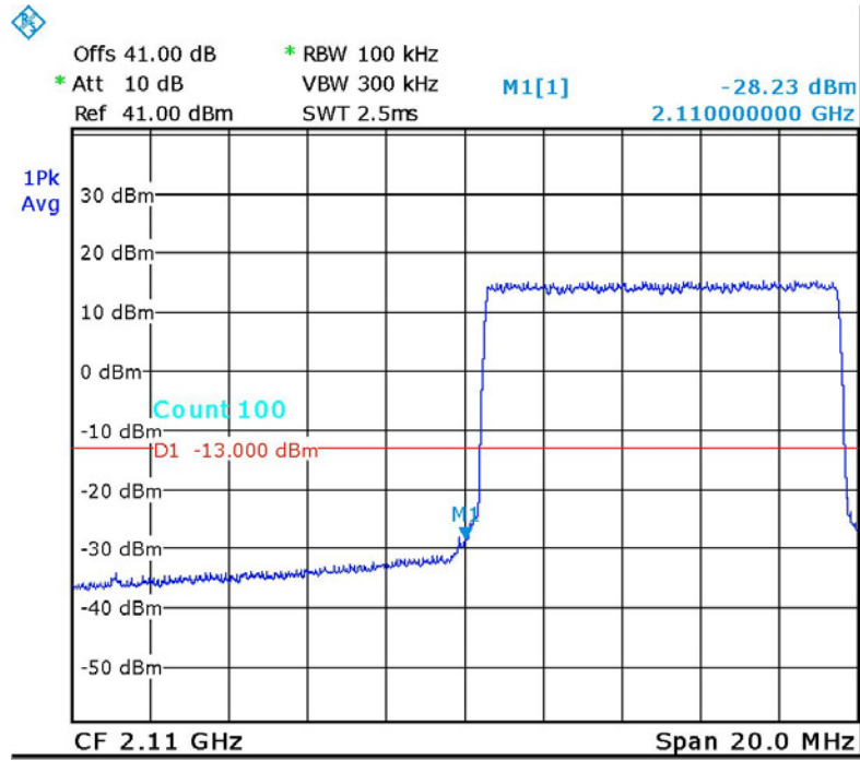
Figure 52. — LTE 64QAM 2115.0 MHz
