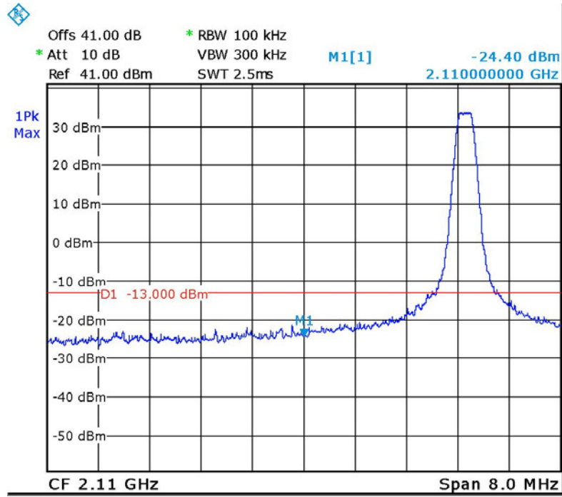
Figure 50. — GSM 2111.2 MHz
