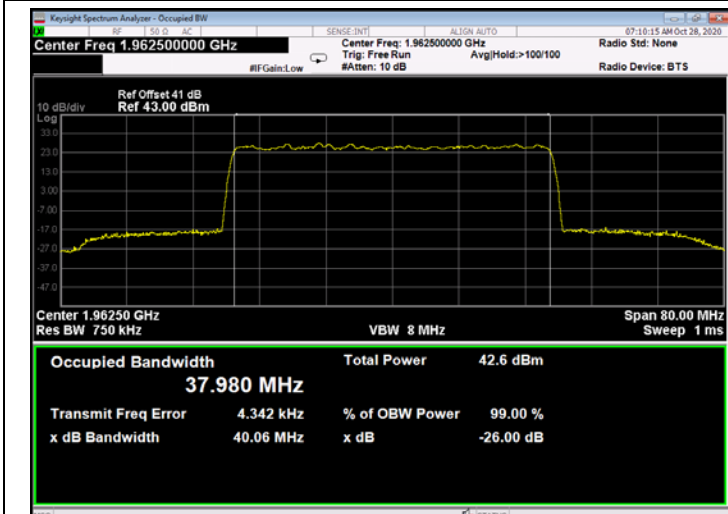
Figure 649: 64QAM 40MHz B.W.; 1962.5MHz, 30kHz - Output
