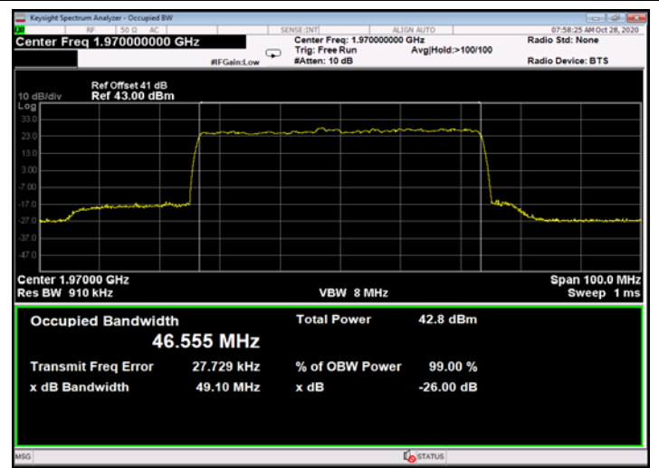
Figure 662: 64QAM 50MHz B.W.; 1970.0MHz, 60kHz - Output
