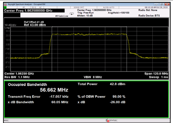
Figure 666: 64QAM 60MHz B.W.; 1962.5MHz, 60kHz - Output
