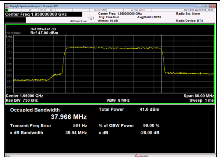
Figure 712: 256QAM 40MHz B.W.; 1950.0MHz, 30kHz - Output
