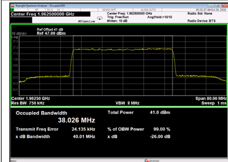
Figure 715: 256QAM 40MHz B.W.; 1962.5MHz, 30kHz - Output
