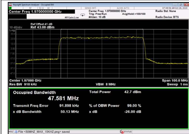
Figure 661: 64QAM 50MHz B.W.; 1970.0MHz, 30kHz - Output
