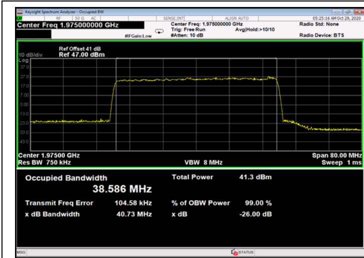
Figure 717: 256QAM 40MHz B.W.; 1975.0MHz, 15kHz - Output
