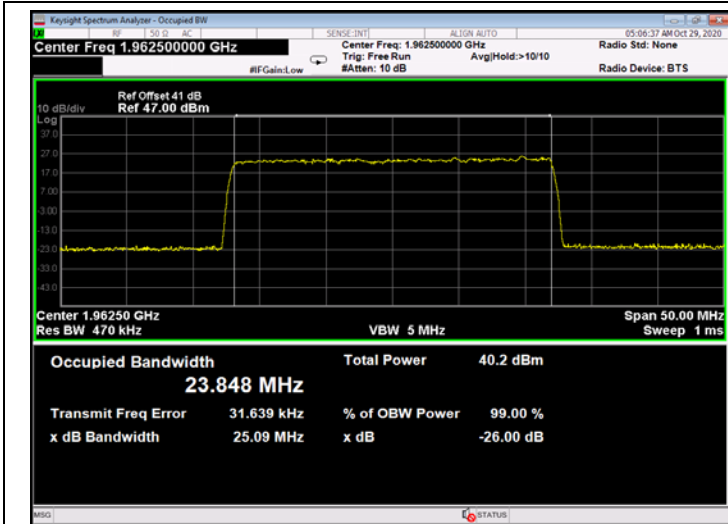
Figure 705: 256QAM 25MHz B.W.; 1962.5MHz, 15kHz - Output
