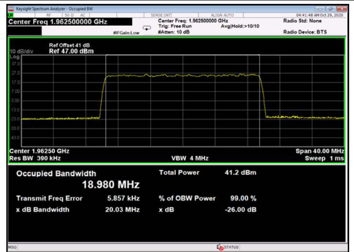
Figure 696: 256QAM 20MHz B.W.; 1962.5MHz, 15kHz - Output
