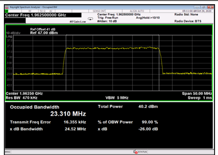
Figure 706: 256QAM 25MHz B.W.; 1962.5MHz, 30kHz - Output
