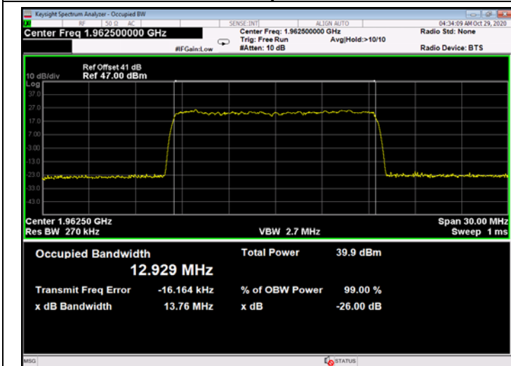
Figure 689: 256QAM 15MHz B.W.; 1962.5MHz, 60kHz - Output
