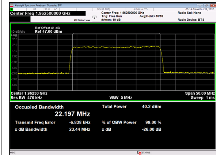
Figure 707: 256QAM 25MHz B.W.; 1962.5MHz, 60kHz - Output
