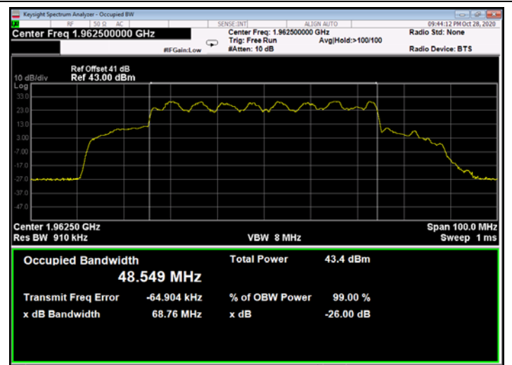
Figure 592: 16QAM 50MHz B.W.; 1962.5MHz, 30kHz - Output
