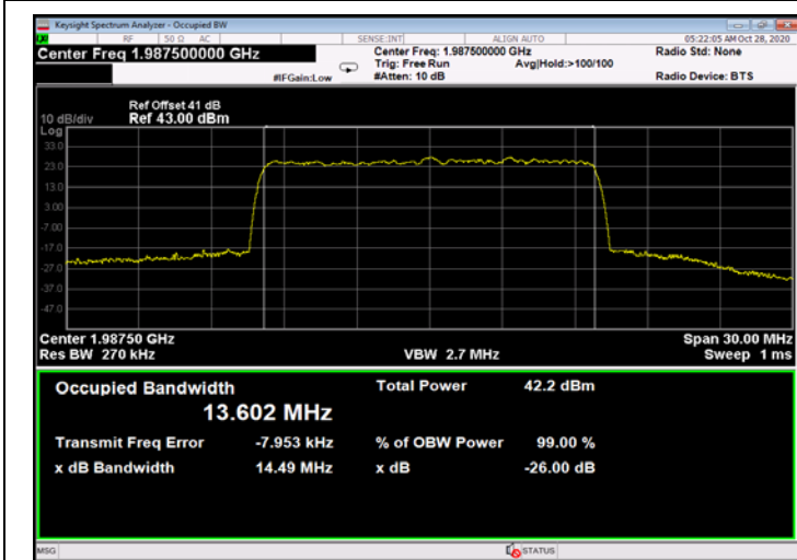
Figure 625: 64QAM 15MHz B.W.; 1987.5MHz, 30kHz - Output
