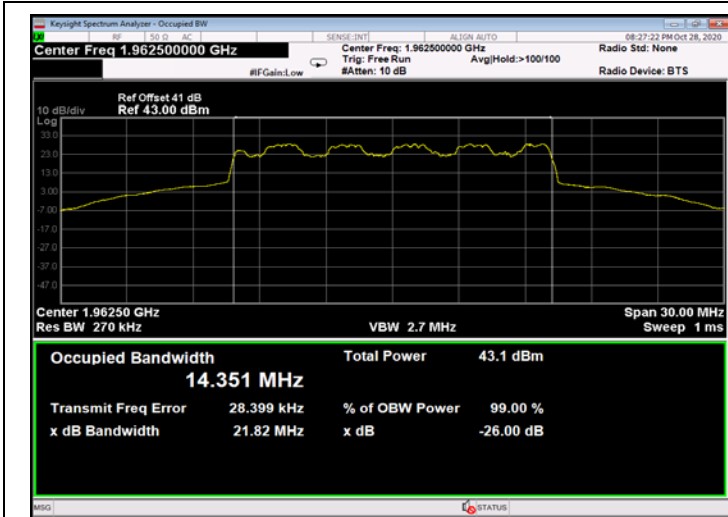
Figure 555: 16QAM 15MHz B.W.; 1962.5MHz, 15kHz - Output
