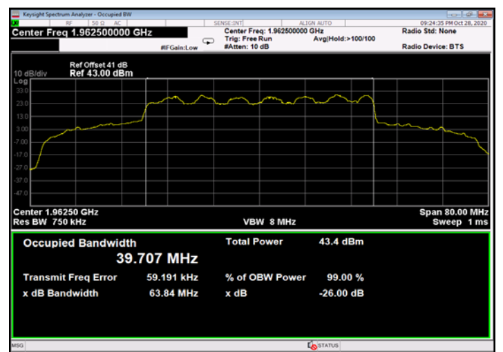
Figure 582: 16QAM 40MHz B.W.; 1962.5MHz, 15kHz - Output
