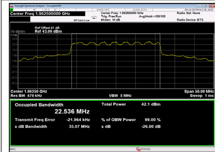
Figure 575: 16QAM 25MHz B.W.; 1962.5MHz, 60kHz - Output
