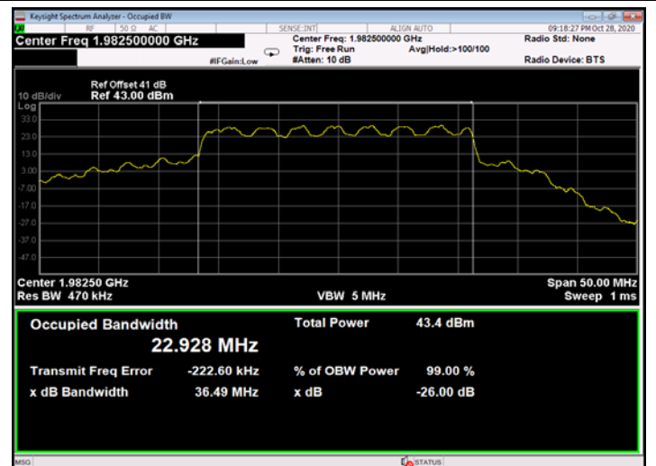
Figure 578: 16QAM 25MHz B.W.; 1982.5MHz, 60kHz - Output
