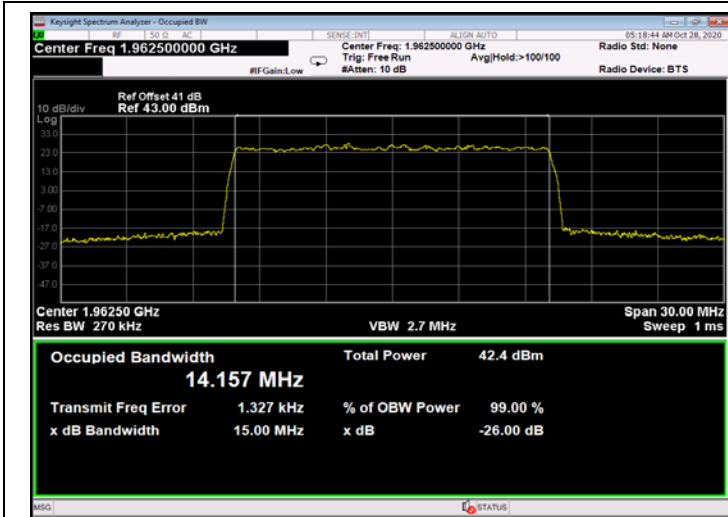
Figure 621: 64QAM 15MHz B.W.; 1962.5MHz, 15kHz - Output
