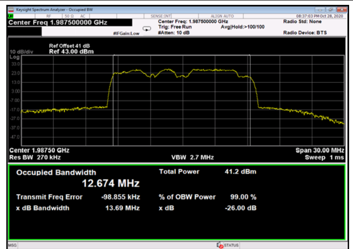
Figure 560: 16QAM 15MHz B.W.; 1987.5MHz, 60kHz - Output
