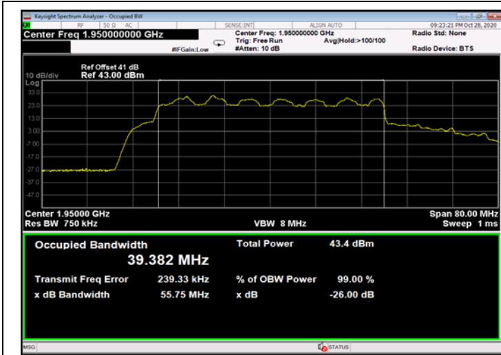
Figure 579: 16QAM 40MHz B.W.; 1950.0MHz, 15kHz - Output
