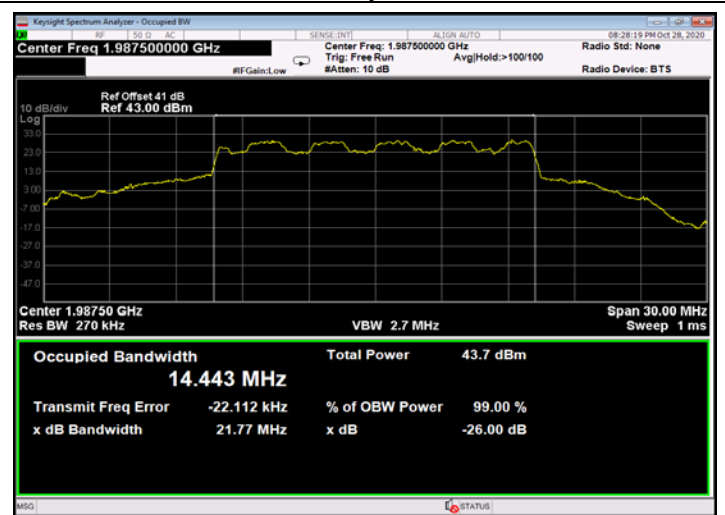
Figure 558: 16QAM 15MHz B.W.; 1987.5MHz, 15kHz - Output
