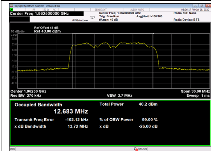
Figure 557: 16QAM 15MHz B.W.; 1962.5MHz, 60kHz - Output
