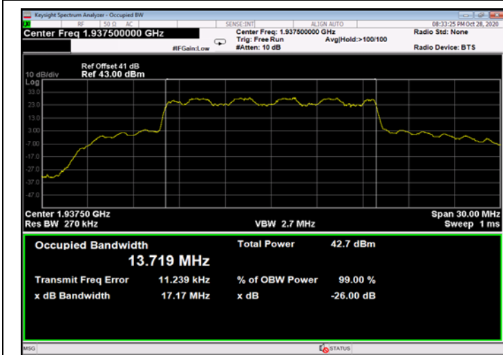
Figure 553: 16QAM 15MHz B.W.; 1937.5MHz, 30kHz - Output
