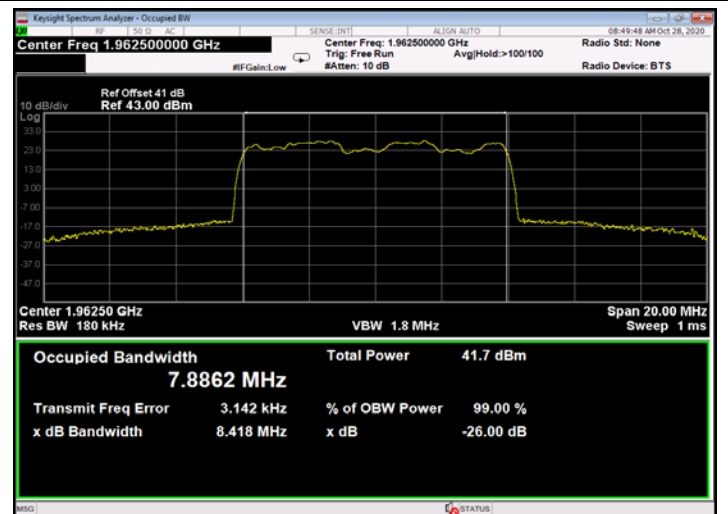
Figure 548: 16QAM 10MHz B.W.; 1962.5MHz, 60kHz - Output
