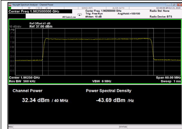
Figure 121: 64QAM 40MHz B.W.; 1962.5MHz, 30kHz
