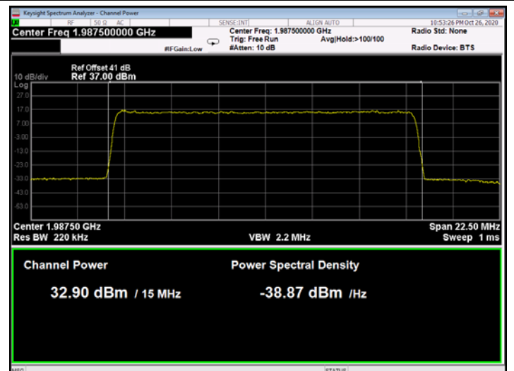
Figure 162: 256QAM 15MHz B.W.; 1987.5MHz, 15kHz
