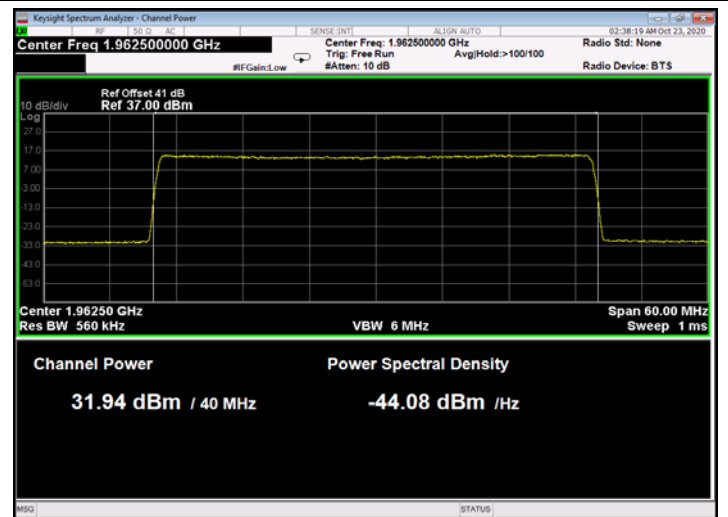
Figure 120: 64QAM 40MHz B.W.; 1962.5MHz, 15kHz
