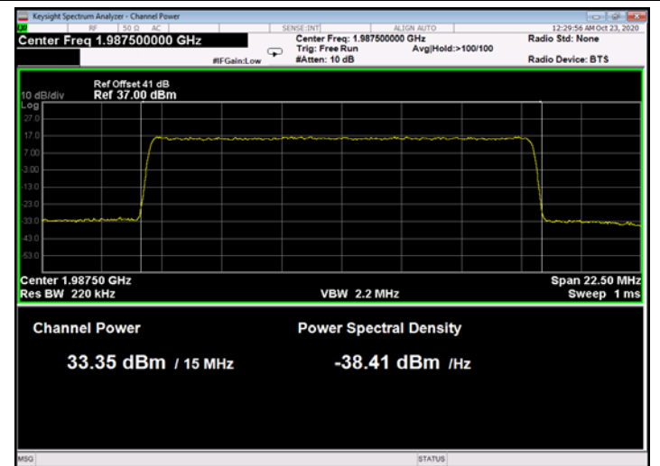
Figure 96: 64QAM 15MHz B.W.; 1987.5MHz, 15kHz
