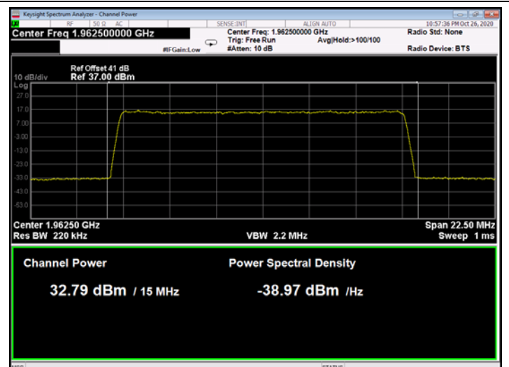
Figure 160: 256QAM 15MHz B.W.; 1962.5MHz, 30kHz
