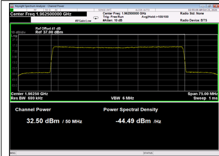
Figure 129: 64QAM 50MHz B.W.; 1962.5MHz, 15kHz
