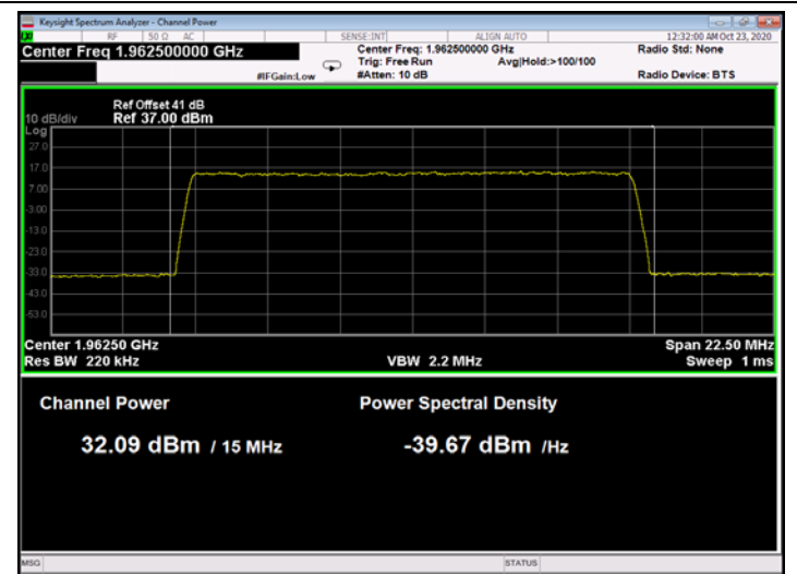
Figure 94: 64QAM 15MHz B.W.; 1962.5MHz, 30kHz
