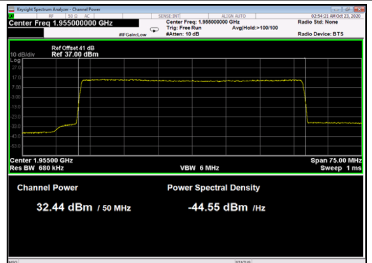
Figure 126: 64QAM 50MHz B.W.; 1955.0MHz, 15kHz
