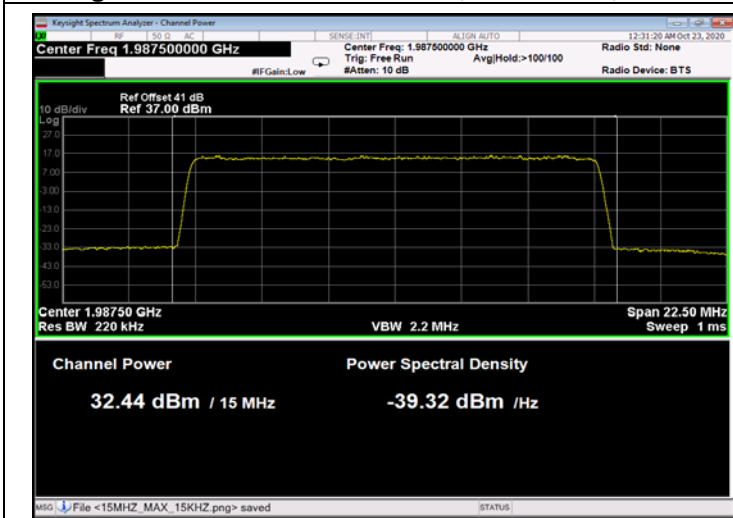
Figure 97: 64QAM 15MHz B.W.; 1987.5MHz, 30kHz
