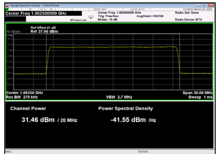
Figure 102: 64QAM 20MHz B.W.; 1962.5MHz, 15kHz
