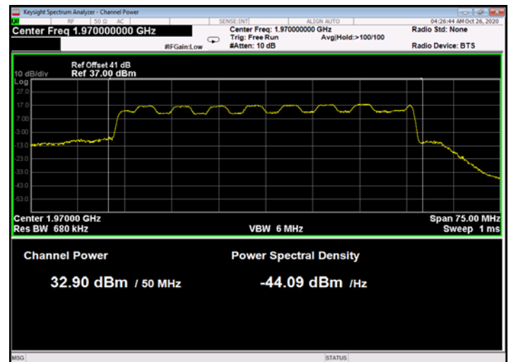
Figure 68: 16QAM 50MHz B.W.; 1970.0MHz, 60kHz
