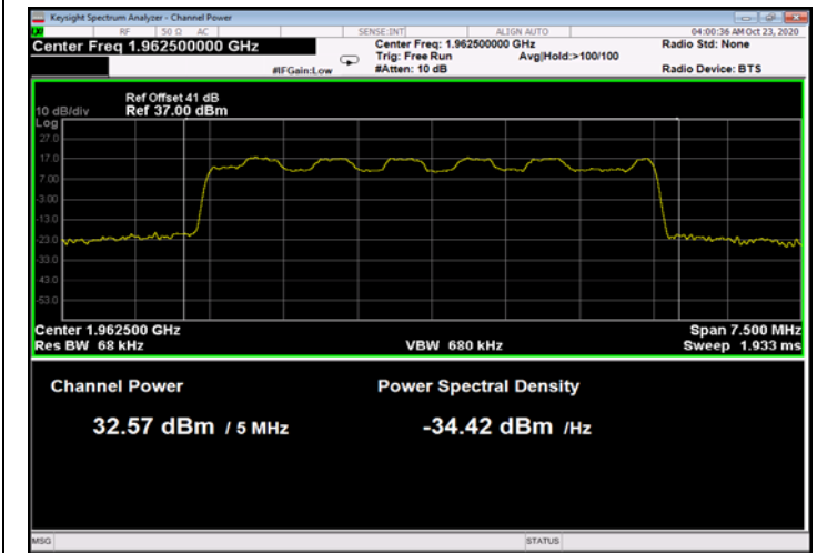
Figure 11: 16QAM 5MHz B.W.; 1962.5MHz, 15kHz
