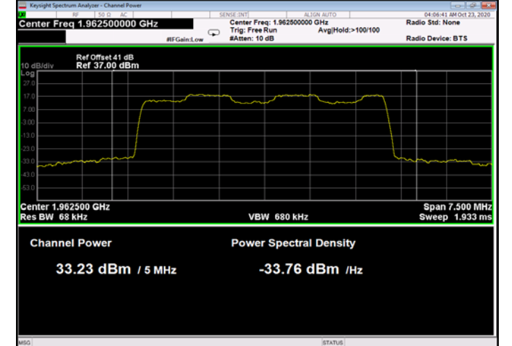
Figure 12: 16QAM 5MHz B.W.; 1962.5MHz, 30kHz
