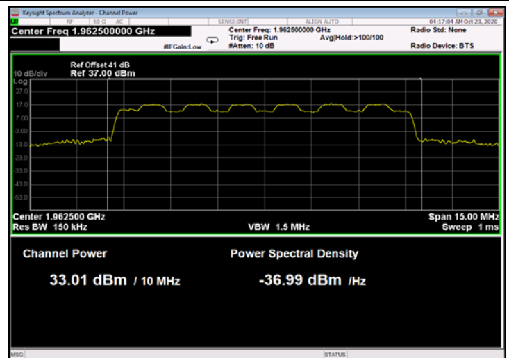
Figure 18: 16QAM 10MHz B.W.; 1962.5MHz, 15kHz
