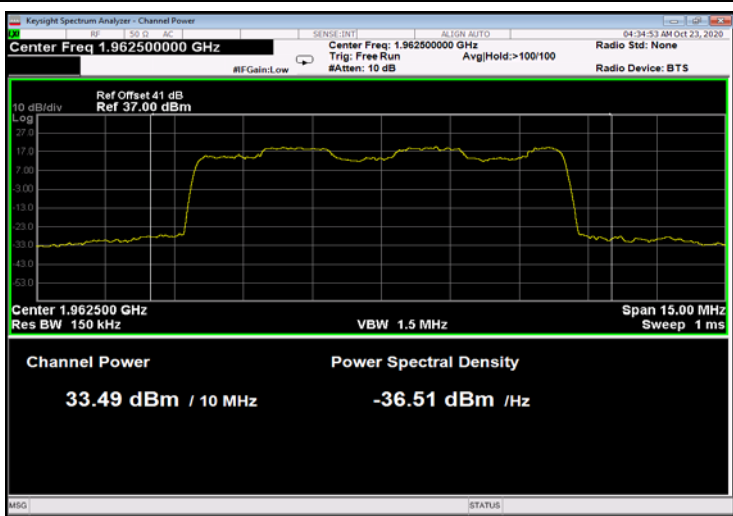
Figure 20: 16QAM 10MHz B.W.; 1962.5MHz, 60kHz
