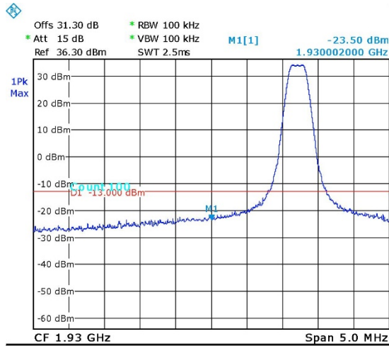
Figure 51. — GSM - 1931.20 MHz
