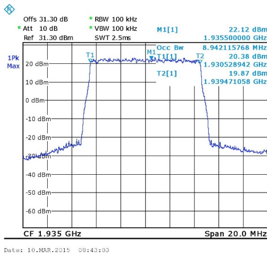
Figure 20. — LTE 64QAM Output 1935.00 MHz
