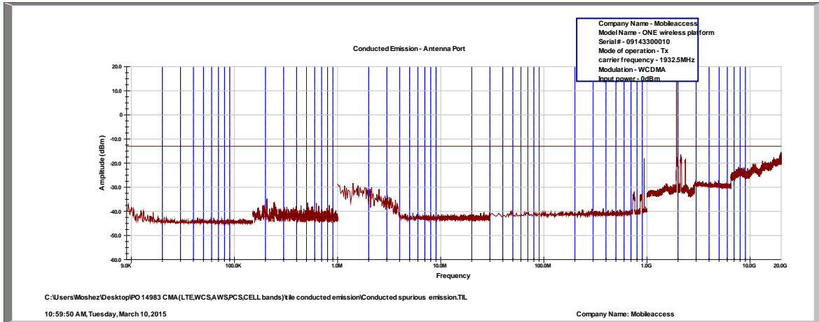
Figure 44. — W-CDMA - 1932.5 MHz
