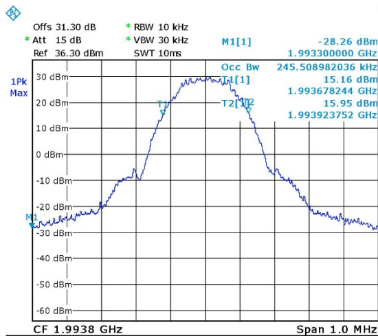
Figure 30. — GSM - Output 1993.80 MHz
