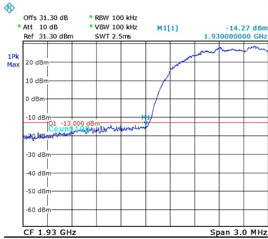
Figure 53. — W-CDMA - 1932.50 MHz
