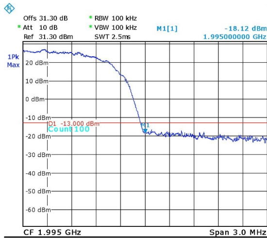
Figure 54. — W-CDMA - 1992.50 MHz
