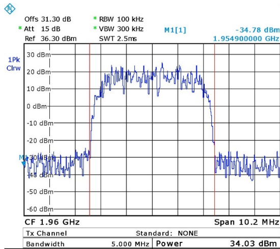
Figure 15. — W-CDMA - 1960.00 MHz
