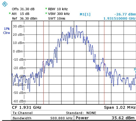
Figure 11. — GSM -1931.20 MHz
