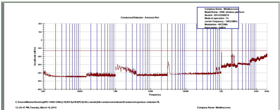
Figure 46. — W-CDMA - 1992.5 MHz
