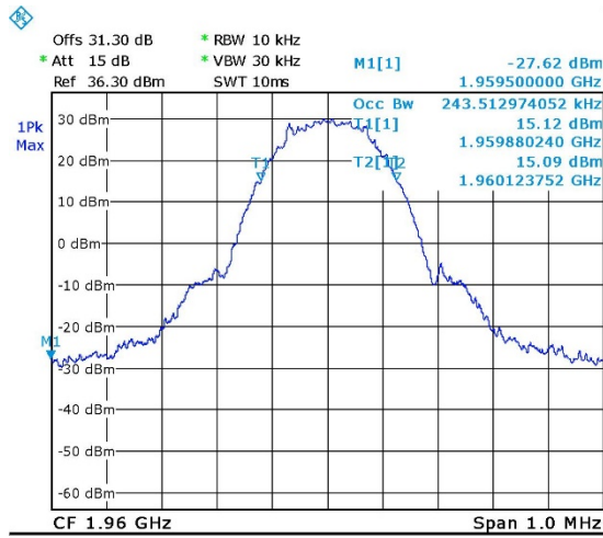
Figure 28. — GSM - Output 1960.00 MHz
