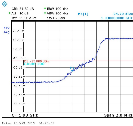
Figure 49. — LTE 64QAM 1935.00 MHz
