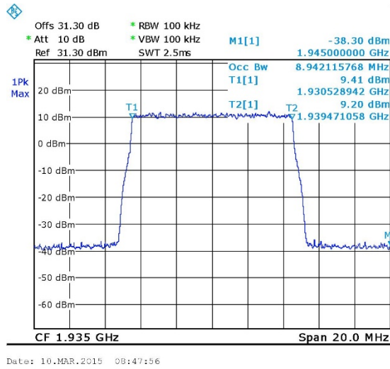
Figure 19. — LTE 64QAM Input 1935.00 MHz
