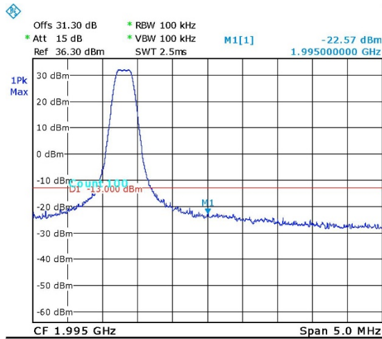
Figure 52. — GSM - 1993.80 MHz
