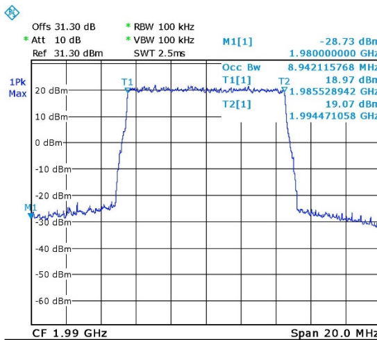
Figure 23. — LTE 64QAM Input 1990.00 MHz
