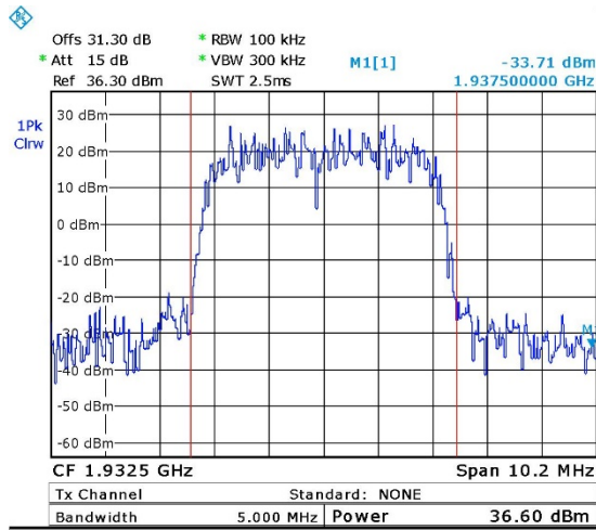
Figure 14. — W-CDMA - 1932.50 MHz
