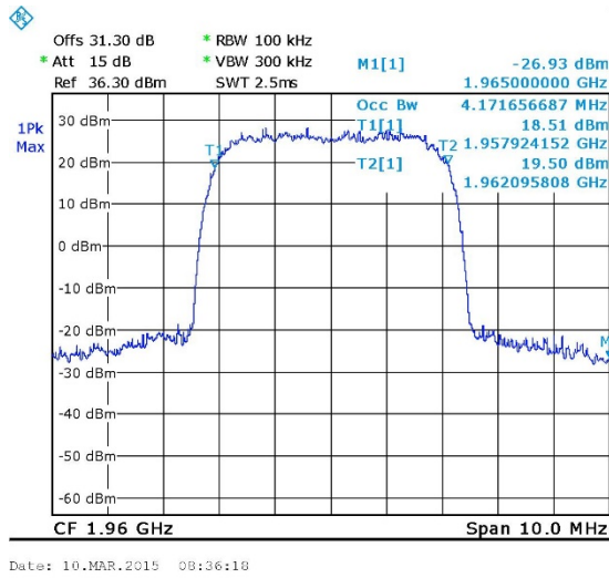
Figure 34. — W-CDMA - Output 1960.00 MHz
