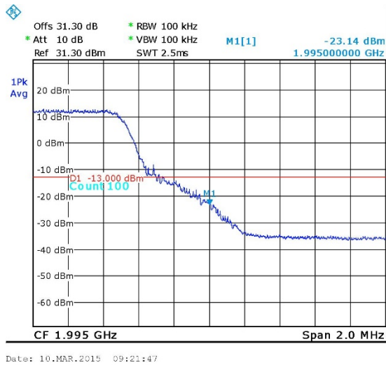
Figure 50. — LTE 64QAM 1990.00 MHz
