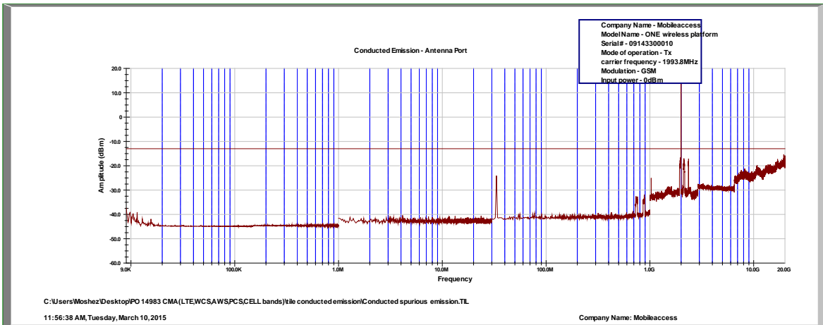
Figure 43. — GSM - 1993.8 MHz
