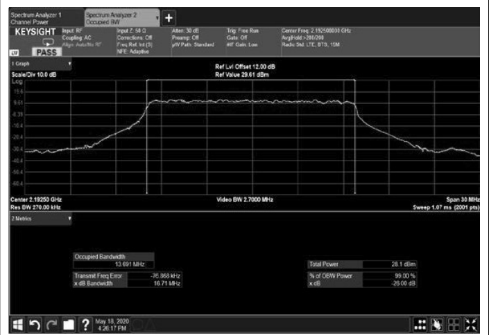
Figure 292: 256QAM 15MHz B.W.; 2192.5MHz, 30kHz Output
