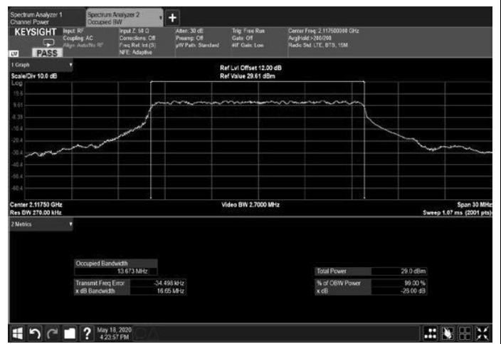
Figure 286: 256QAM 15MHz B.W.; 2117.5MHz, 30kHz Output
