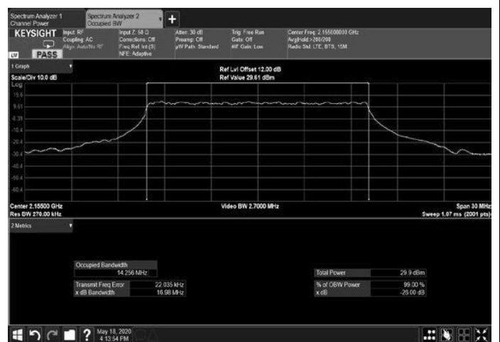
Figure 288: 256QAM 15MHz B.W.; 2155.0MHz, 15kHz Output
