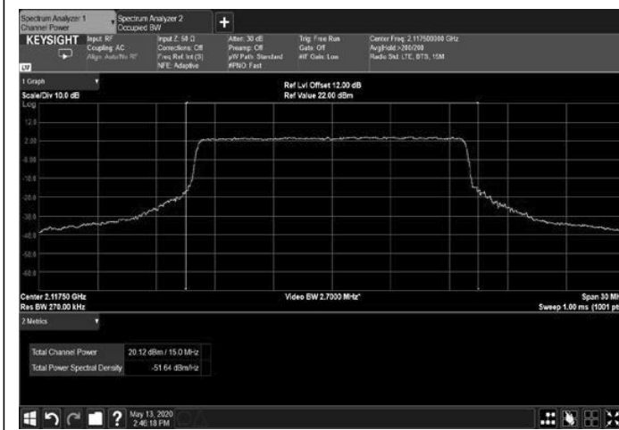
Figure 89: 256QAM 15MHz B.W.; 2117.5MHz, 30kHz
