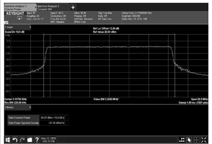
Figure 88: 256QAM 15MHz B.W.; 2117.5MHz, 15Hz
