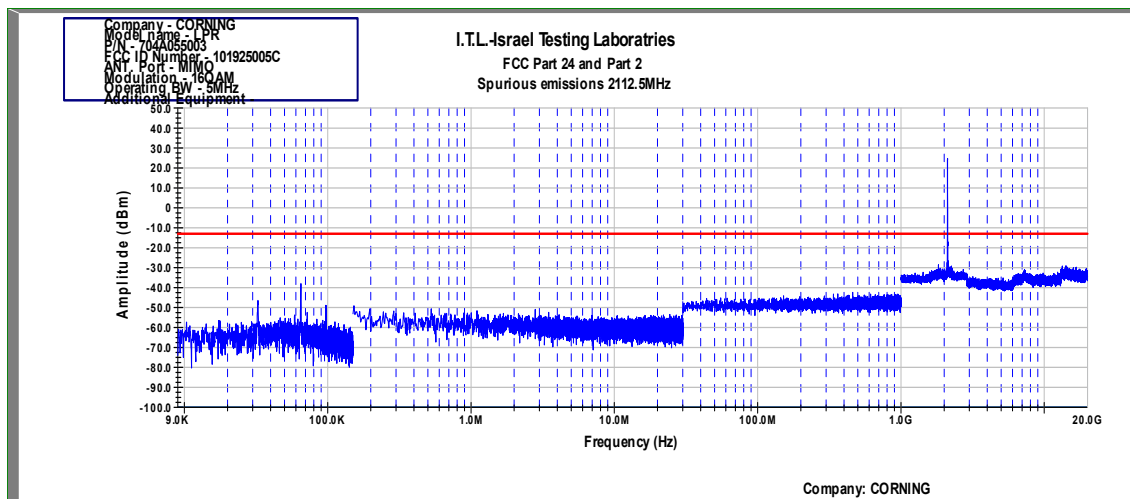
Figure 126 Spurious Emissions at Antenna Terminals 16QAM, MIMO, 5 MHz (Low)
