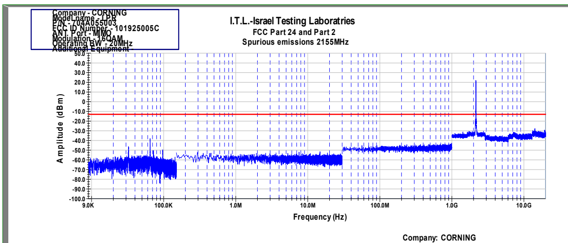
Figure 136 Spurious Emissions at Antenna Terminals 16QAM, MIMO, 20 MHz (Mid)
