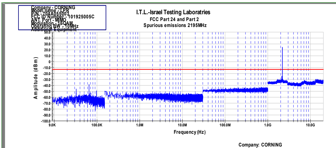
Figure 131 Spurious Emissions at Antenna Terminals 16QAM, MIMO, 10 MHz (High)
