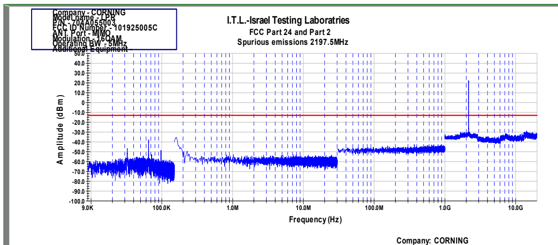
Figure 128 Spurious Emissions at Antenna Terminals 16QAM, MIMO, 5 MHz (High)
