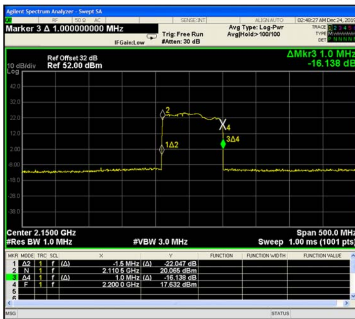
Figure 193. — Out-of-Band Rejection Plot 20MHz
