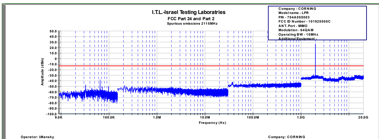
Figure 141 Spurious Emissions at Antenna Terminals 64QAM, MIMO, 10 MHz (Low)
