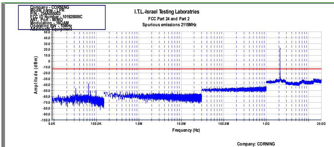
Figure 129 Spurious Emissions at Antenna Terminals 16QAM, MIMO, 10 MHz (Low)
