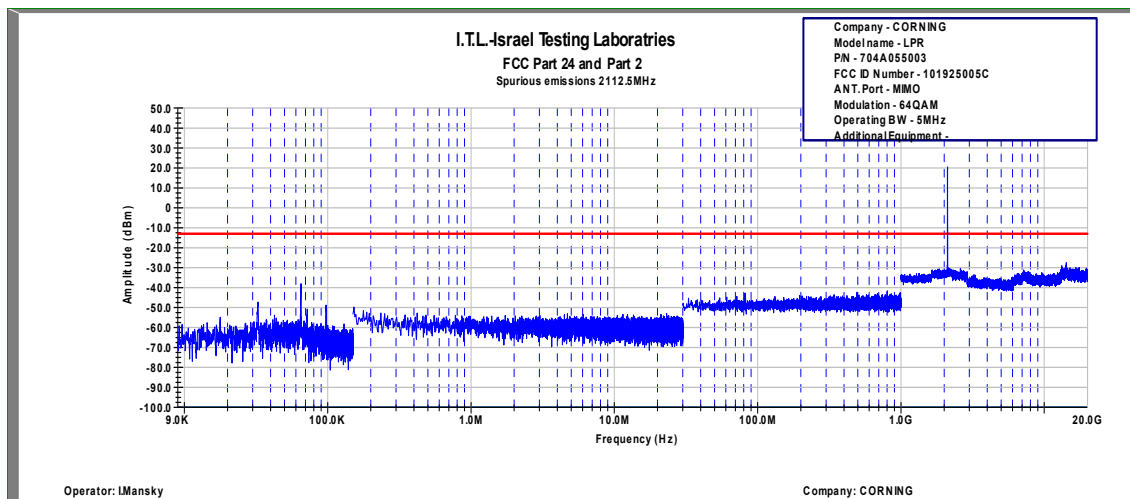
Figure 138 Spurious Emissions at Antenna Terminals 64QAM, MIMO, 5 MHz (Low)
