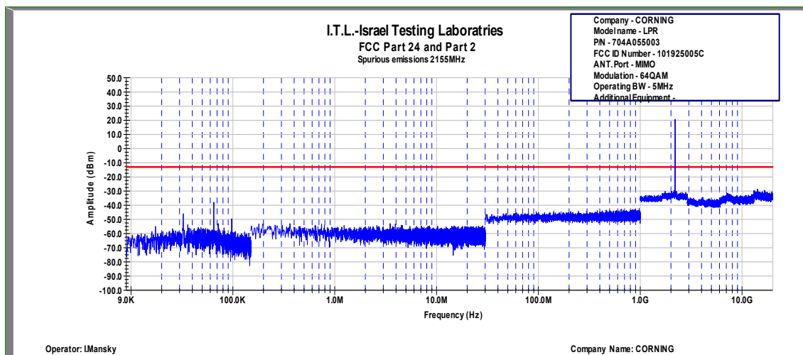
Figure 139 Spurious Emissions at Antenna Terminals 64QAM, MIMO, 5 MHz (Mid)
