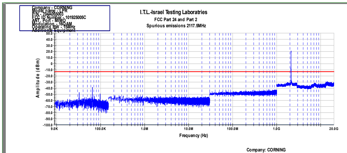
Figure 132 Spurious Emissions at Antenna Terminals 16QAM, MIMO, 15 MHz (Low)
