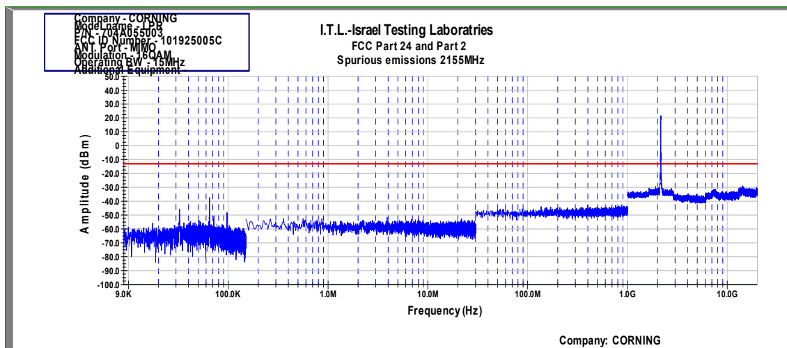
Figure 133 Spurious Emissions at Antenna Terminals 16QAM, MIMO, 15MHz (Mid)
