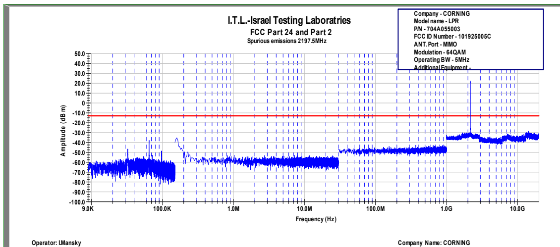
Figure 140 Spurious Emissions at Antenna Terminals 64QAM, MIMO, 5 MHz (High)
