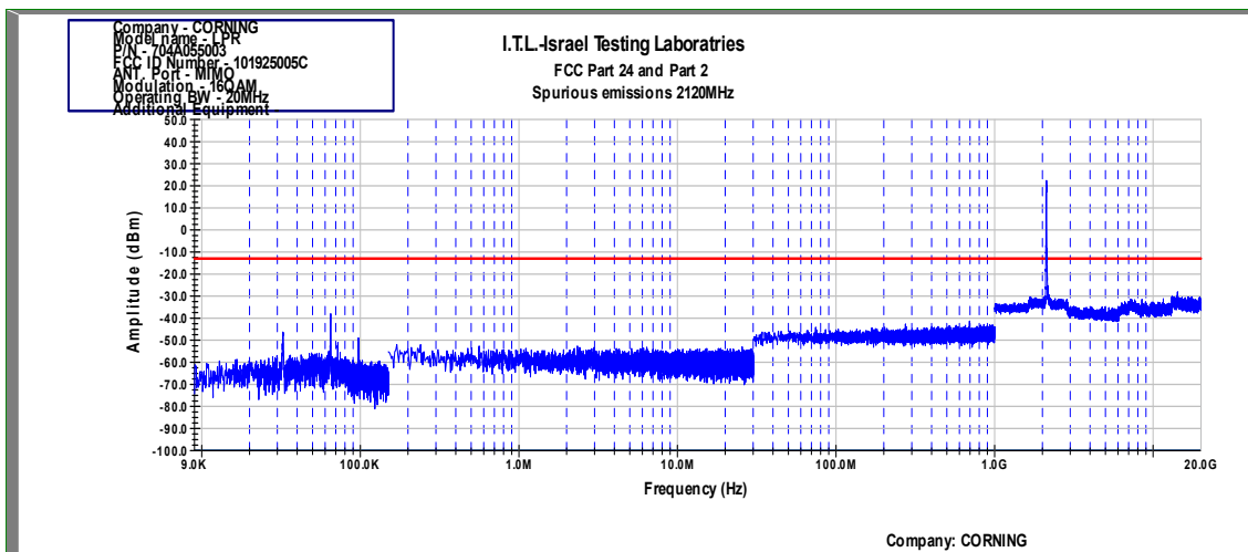
Figure 135 Spurious Emissions at Antenna Terminals 16QAM, MIMO, 20 MHz (Low)
