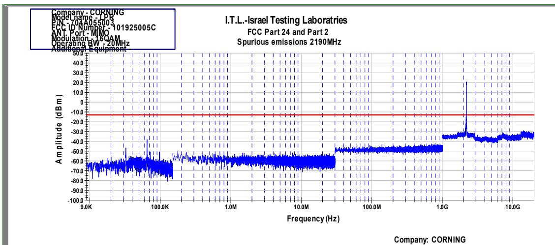
Figure 137 Spurious Emissions at Antenna Terminals 16QAM, MIMO, 20 MHz (High)
