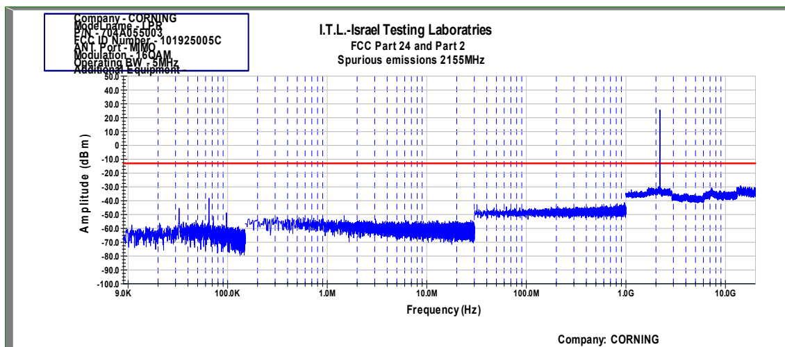
Figure 127 Spurious Emissions at Antenna Terminals 16QAM, MIMO, 5 MHz (Mid)
