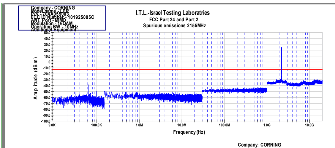
Figure 130 Spurious Emissions at Antenna Terminals 16QAM, MIMO, 10 MHz (Mid)
