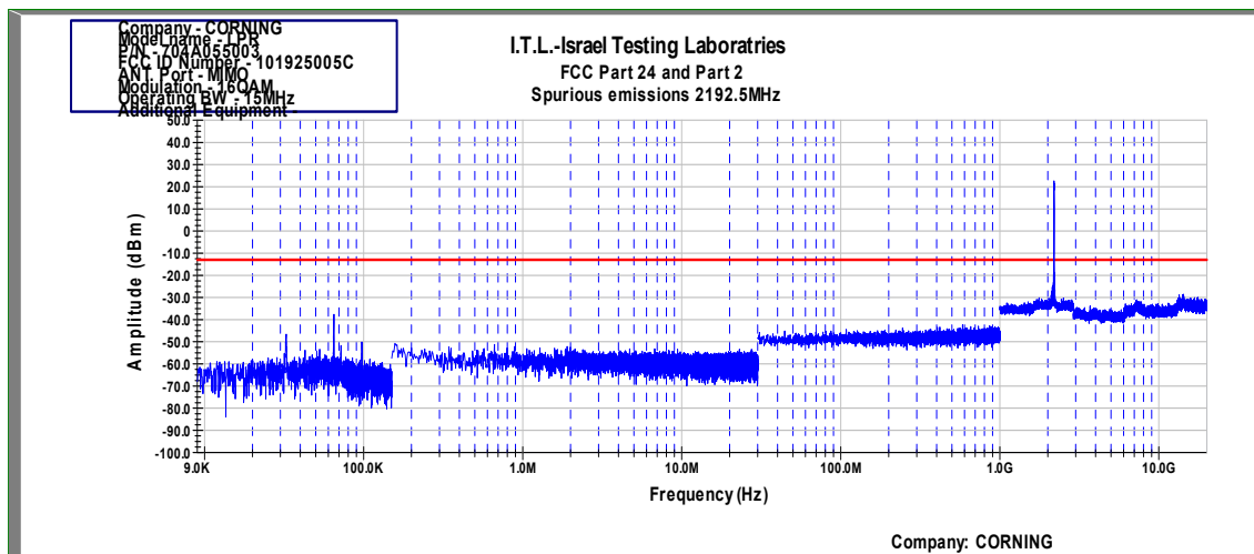
Figure 134 Spurious Emissions at Antenna Terminals 16QAM, MIMO, 15MHz (High)
