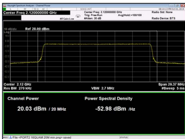
Figure 58 20MHz BW, 2120MHz
