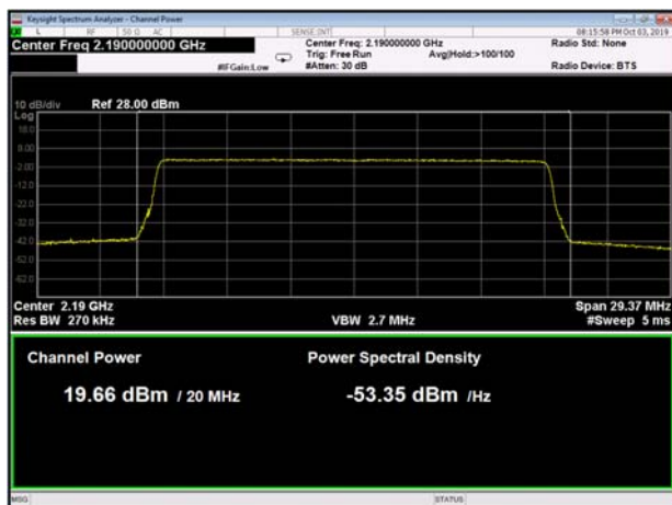
Figure 60 20MHz BW, 2190MHz
