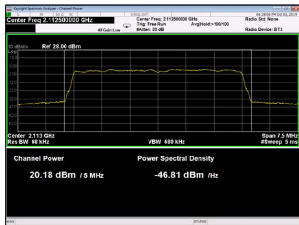
Figure 25 5MHz BW, 2112.5MHz
