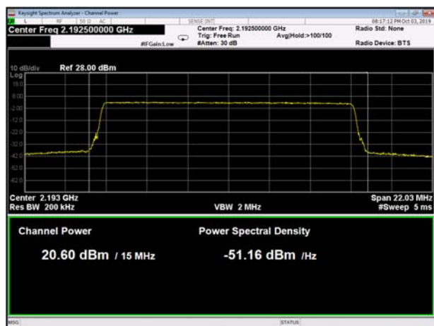
Figure 57 15MHz BW, 2192.5MHz
