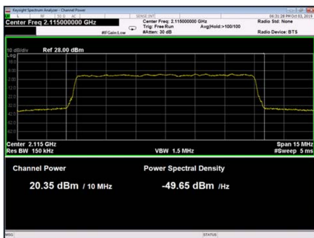
Figure 28 10MHz BW, 2115MHz
