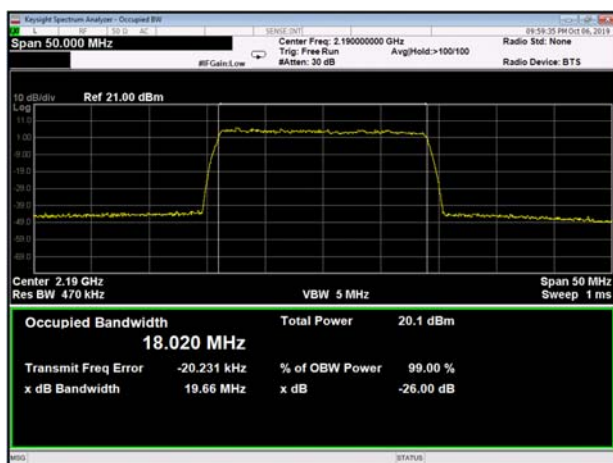
Figure 101 20MHz BW, 2190MHz
