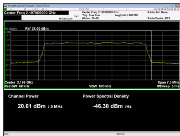
Figure 27 5MHz BW, 2197.5MHz
