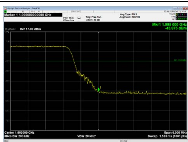
Figure 178 20MHz BW, 1985MHz
