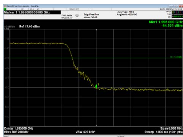
Figure 186 20MHz BW, 1985MHz
