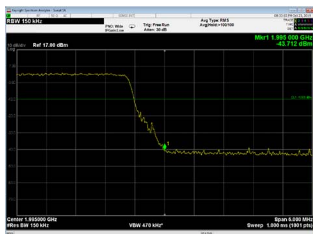
Figure 184 15MHz BW, 1987.5MHz
