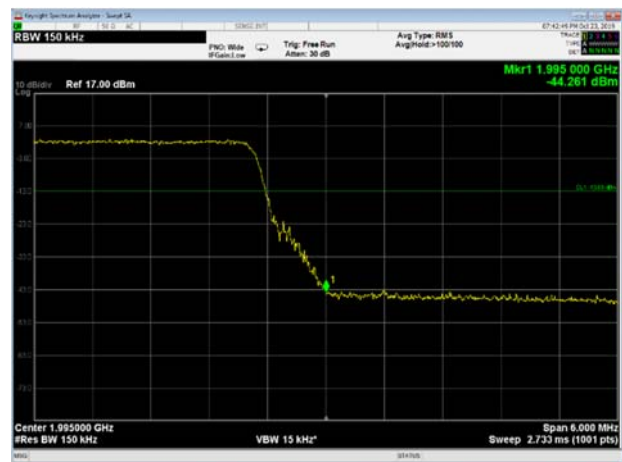
Figure 176 15MHz BW, 1987.5MHz
