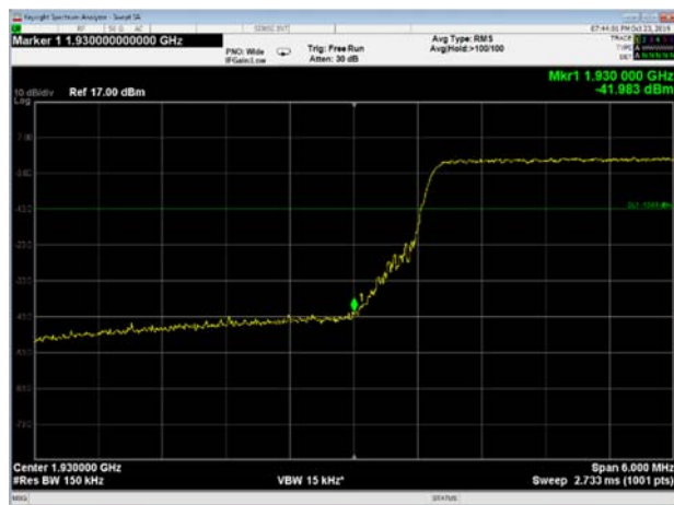
Figure 175 15MHz BW, 1937.5MHz
