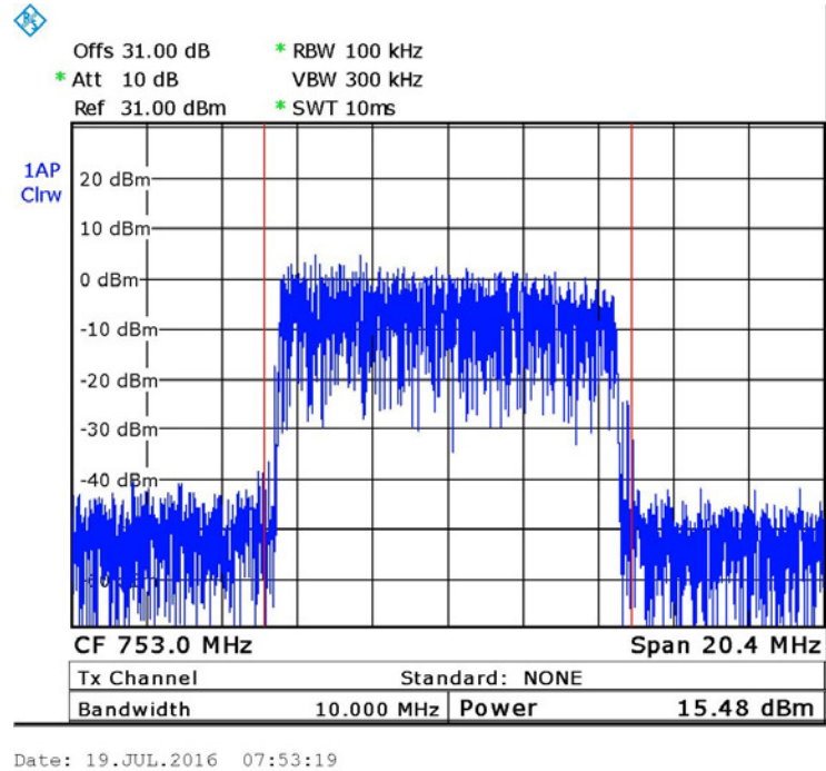
Figure 19. — QPSK 753 MHz
