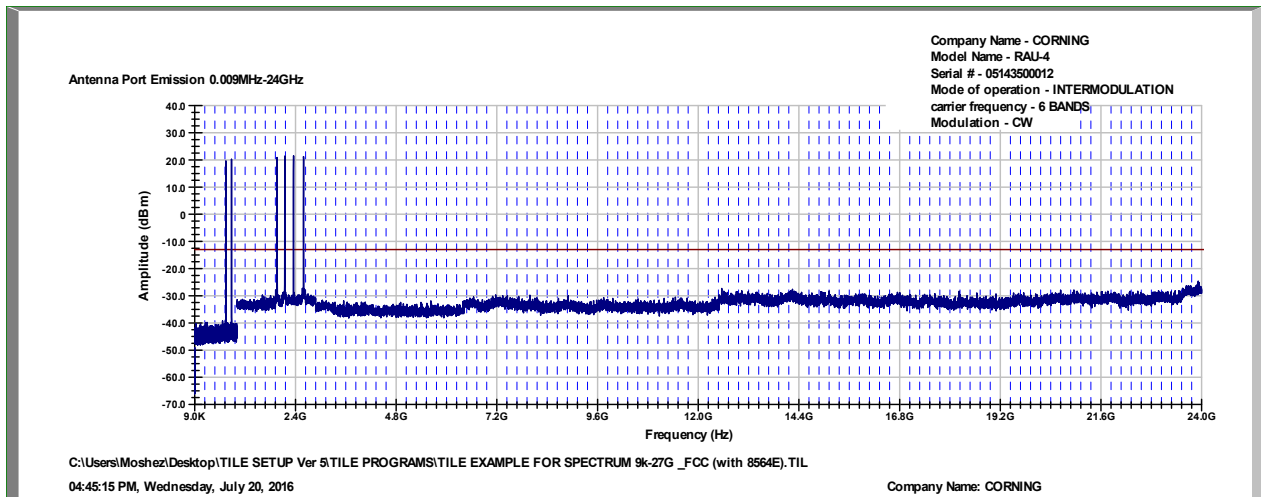
Figure 61 Intermodulation Conducted
