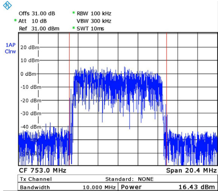
Figure 13. — 64QAM 753 MHz
