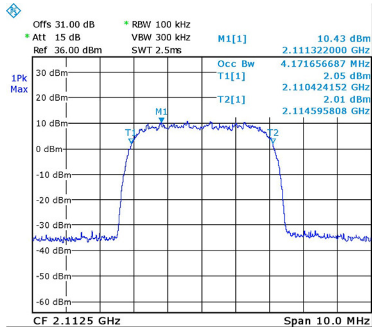
Figure 34. — W-CDMA (2112.5 MHz) IN
