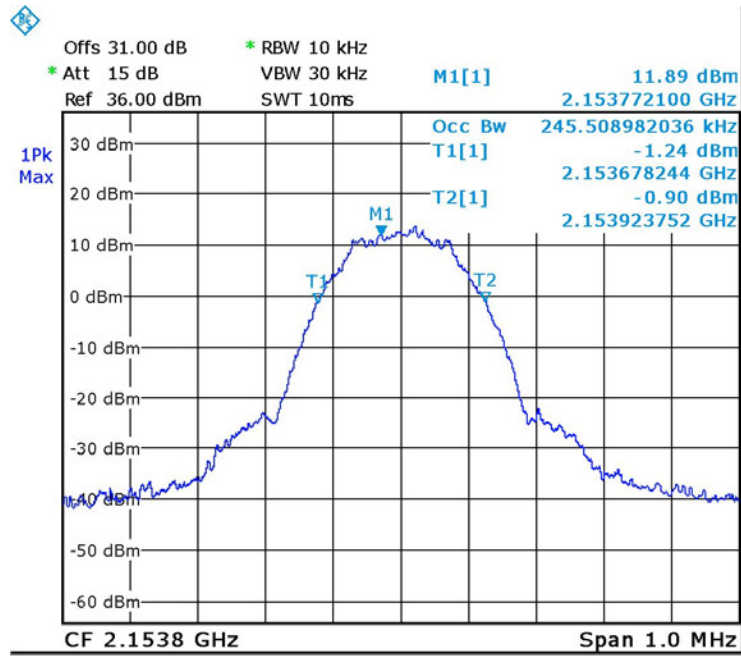
Figure 32. — GSM (2153.8 MHz) IN
