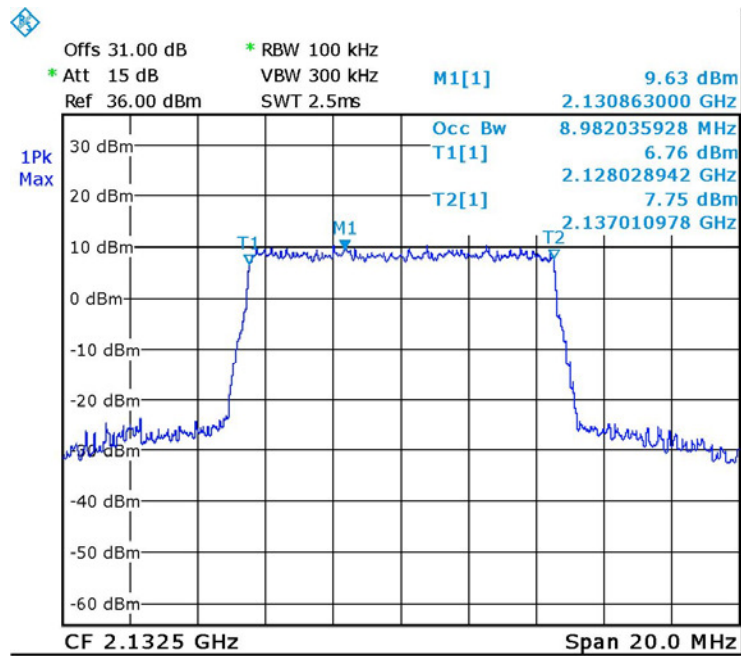
Figure 24. — LTE 64QAM (2132.5MHz) IN
