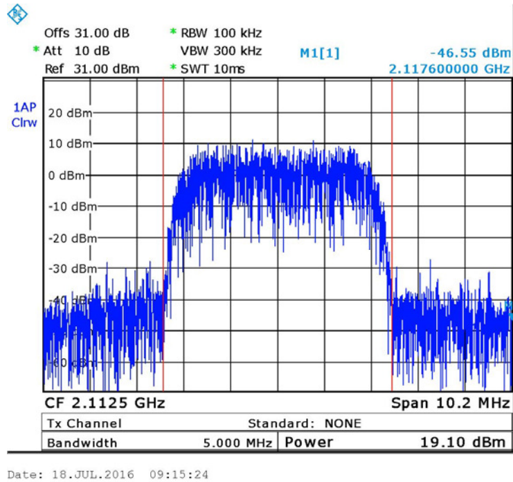
Figure 17. — W-CDMA (2112.5 MHz)
