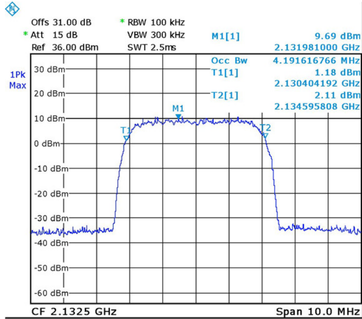
Figure 36. — W-CDMA (2132.5MHz) IN
