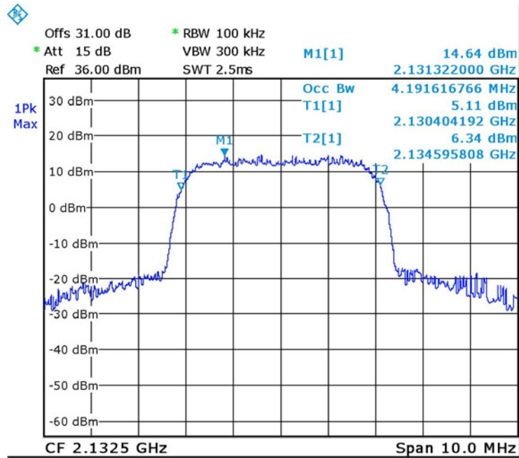
Figure 37. — W-CDMA (2132.5MHz) OUT
