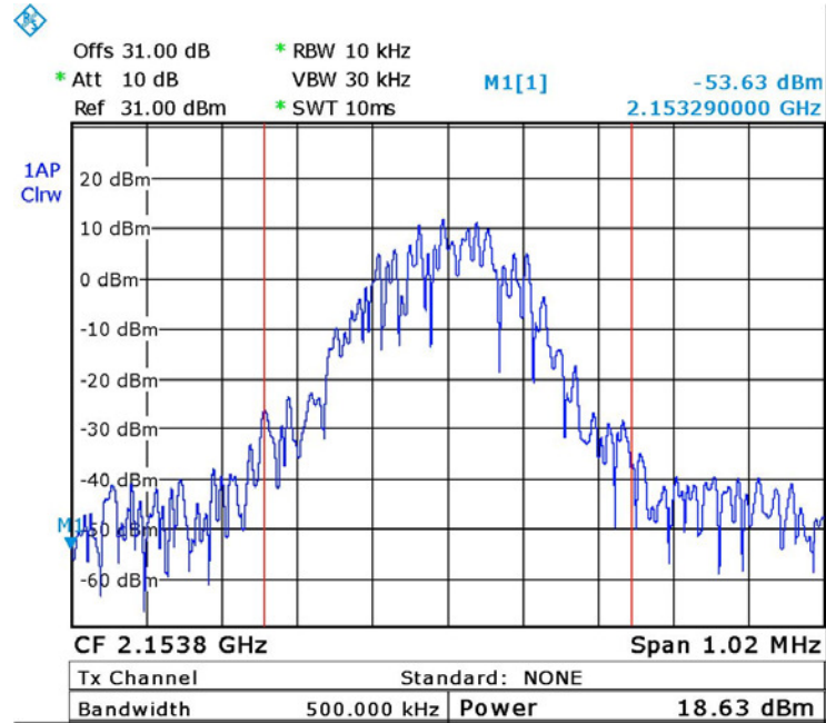
Figure 13. — GSM (2153.8 MHz)
