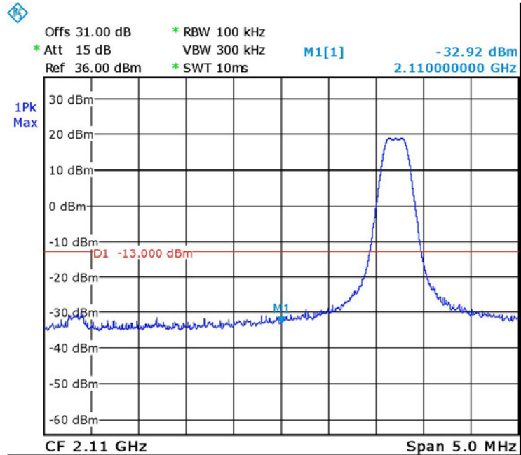
Figure 52. — GSM 2111.2 MHz
