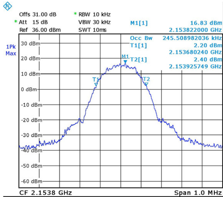
Figure 33. — GSM (2153.8 MHz) OUT
