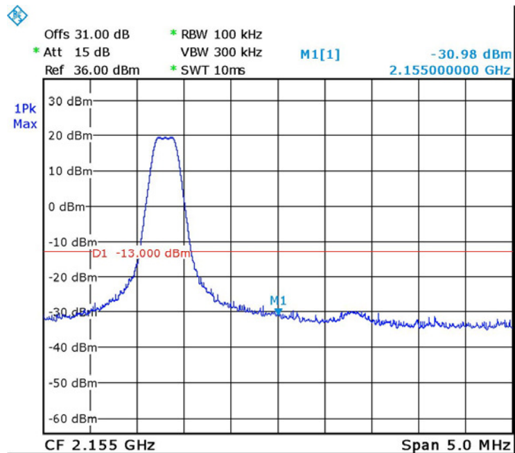
Figure 53. — GSM 2153.8 MHz
