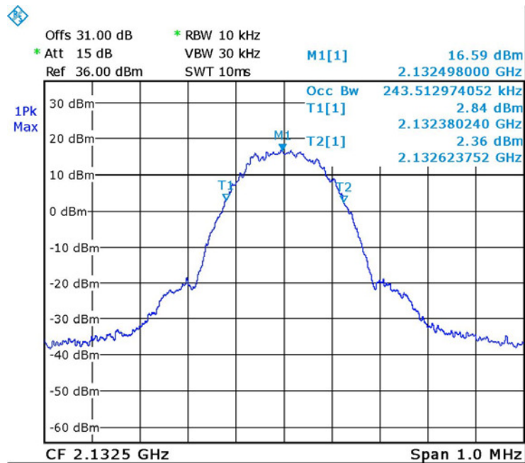
Figure 30. — GSM (2132.5MHz) IN
