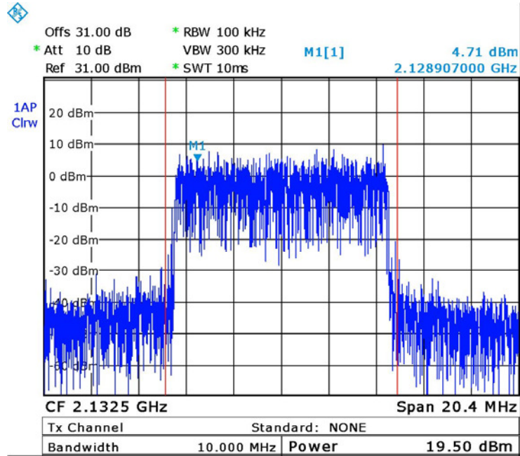
Figure 15. — LTE 64QAM (2132.50MHz)
