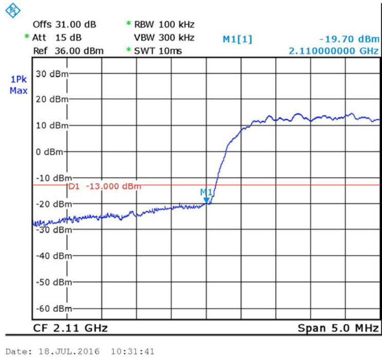
Figure 56. — W-CDMA 2112.5 MHz
