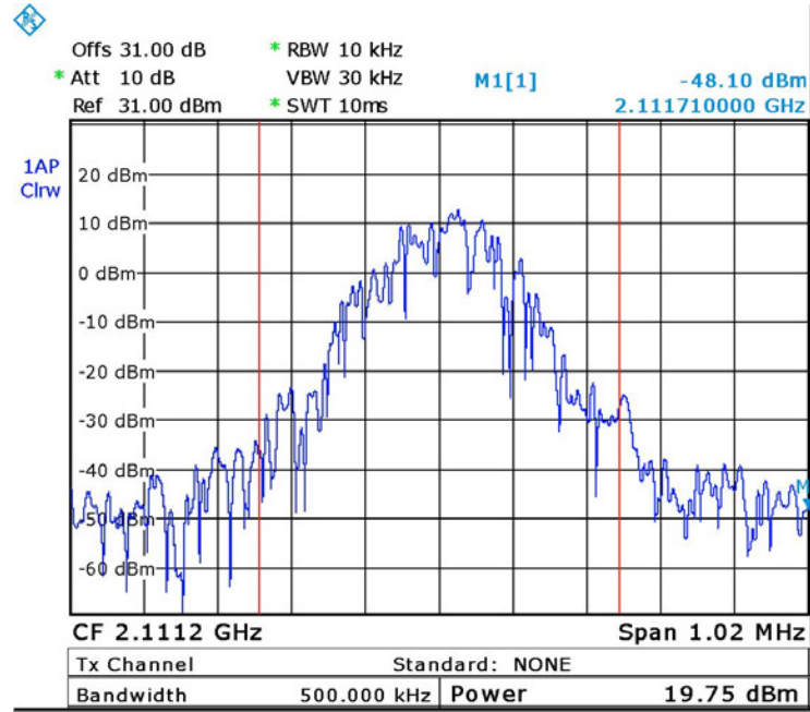
Figure 11. — GSM (2111.2 MHz)
