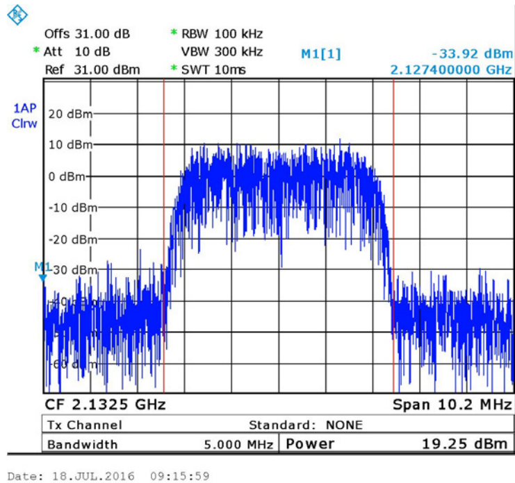
Figure 18. — W-CDMA (2132.5 MHz)
