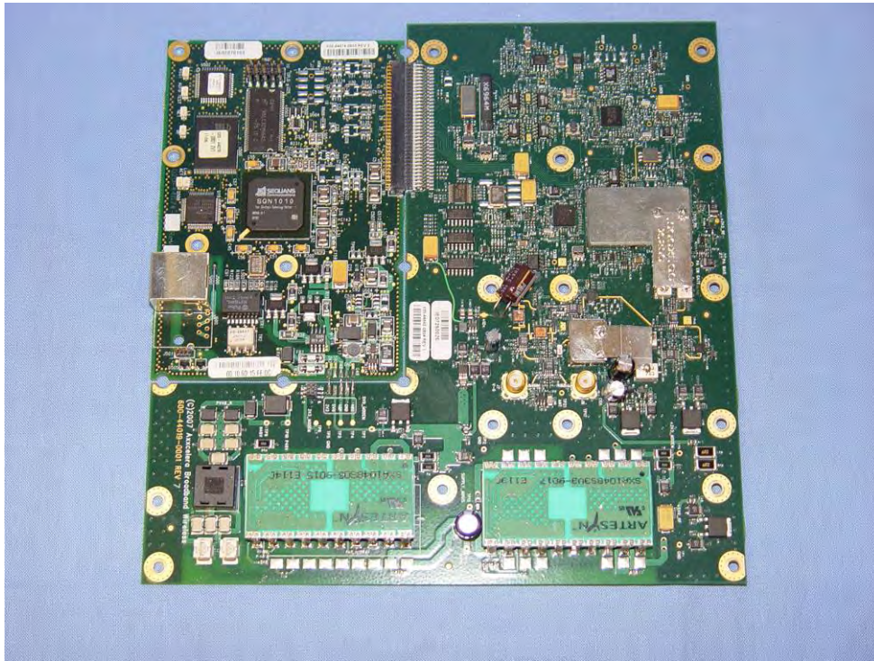
RF and Processor Assembly Top
