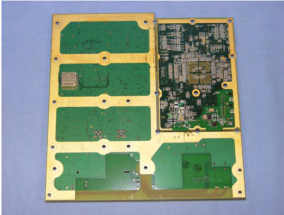
RF and Processor Assembly Bottom
