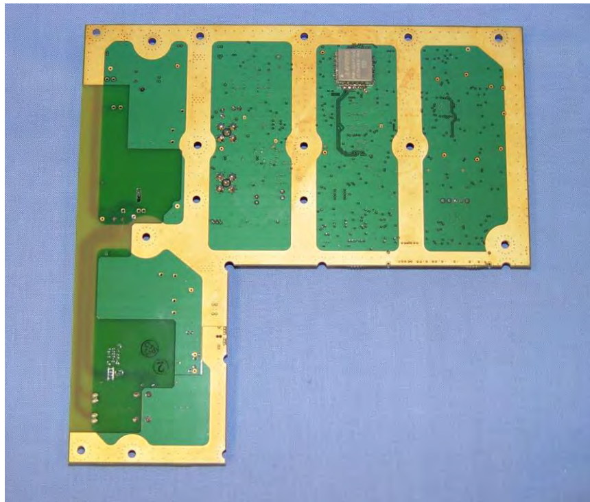
RF Assembly Bottom
