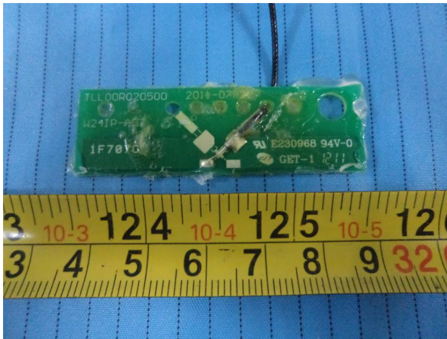
EUT – Antenna Board 2 Top View
