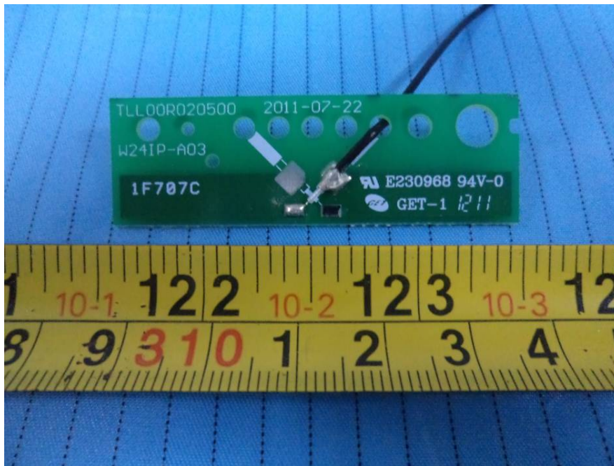
EUT – Antenna Board 1 Top View
