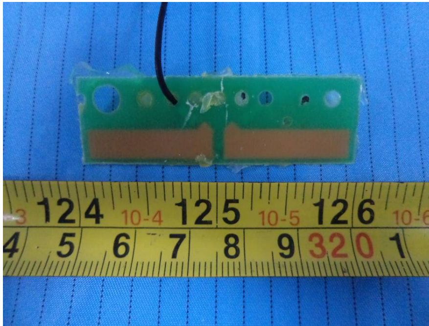
EUT – Antenna Board 2 Bottom View
