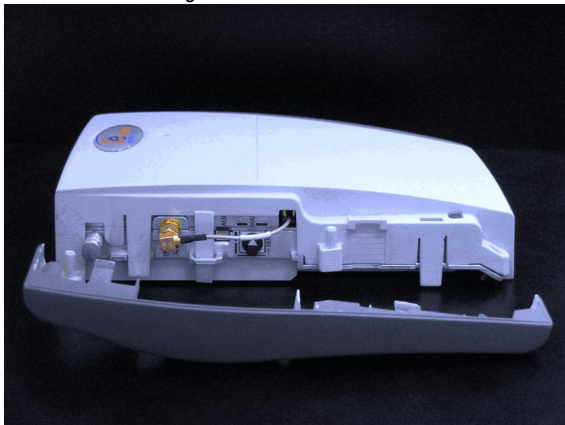
Figure 7– Left side view, with side cover removed
