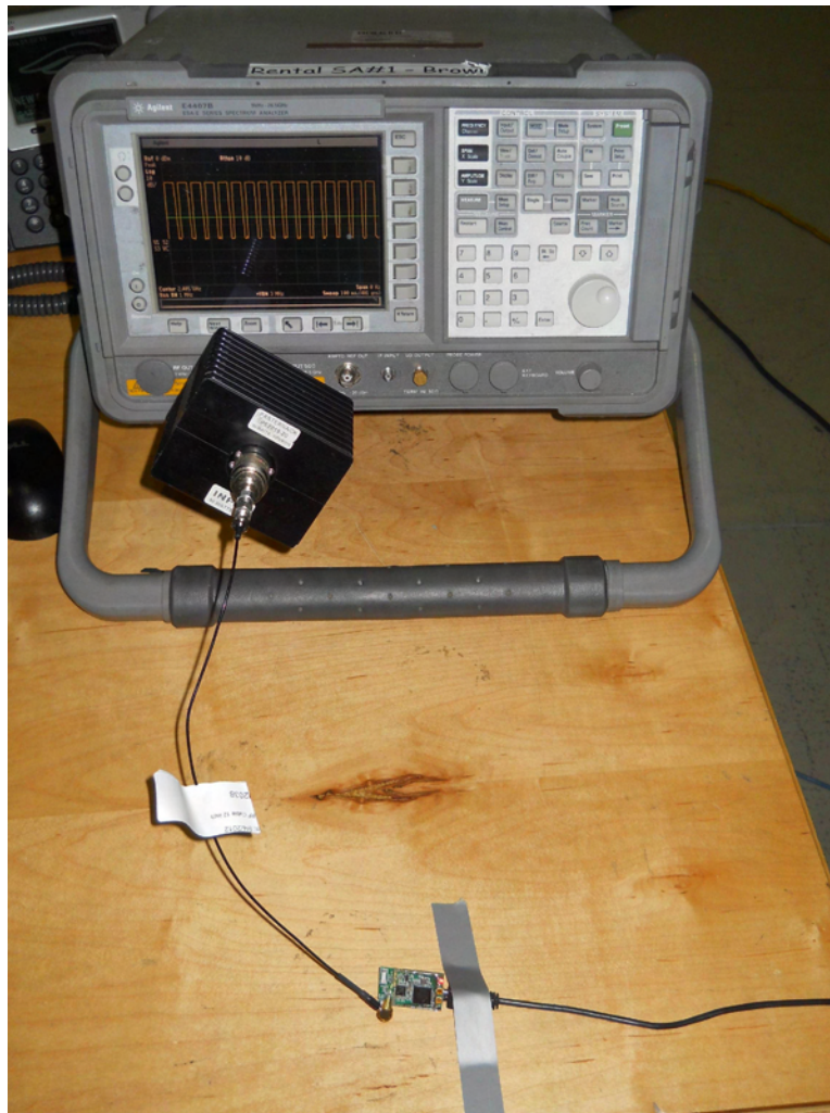
Conducted Emissions
