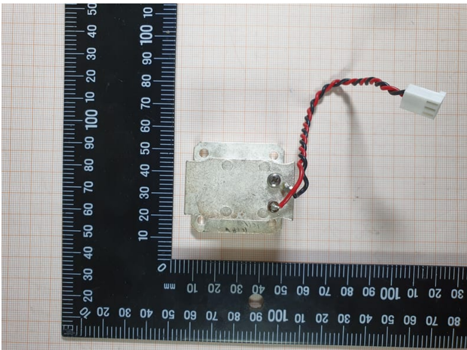
Photo 12: 24 GHz transceiver
