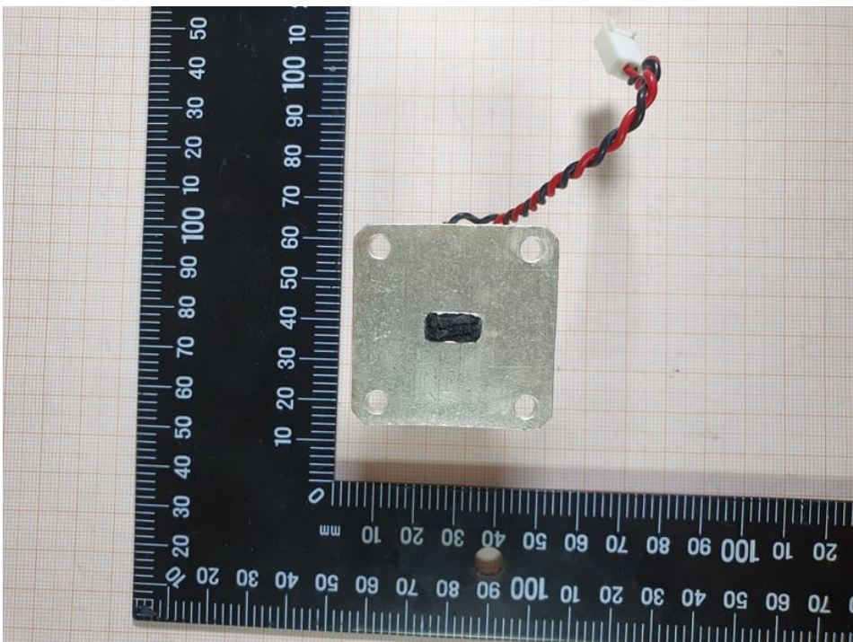
Photo 8: 24 GHz transceiver
