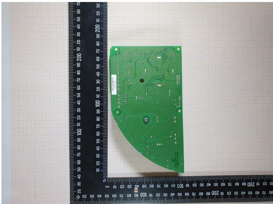
Photo 4: Bottom PCB
