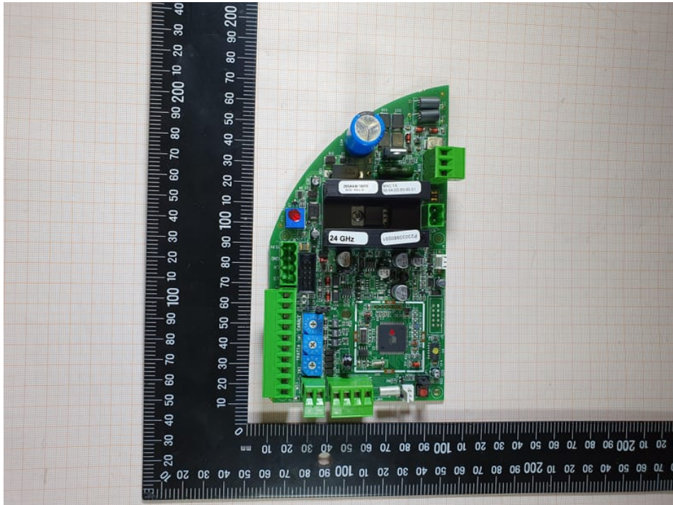
Photo 3: Top PCB
