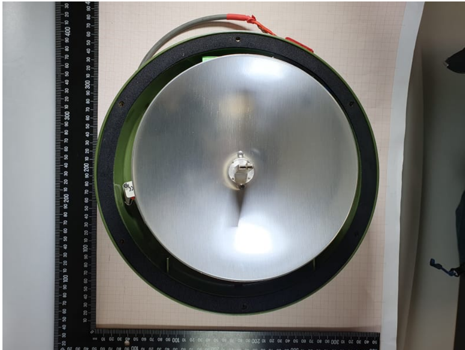
Photo 1: Parabolic reflector
