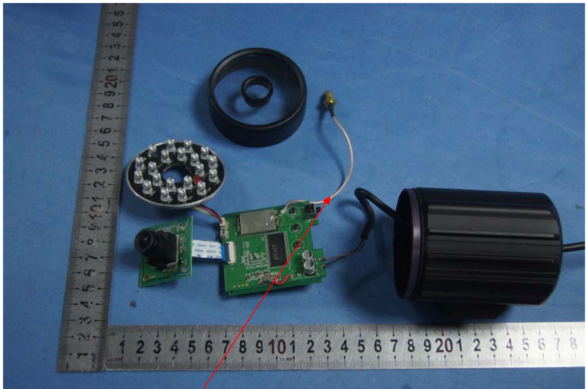
Antenna Connector
