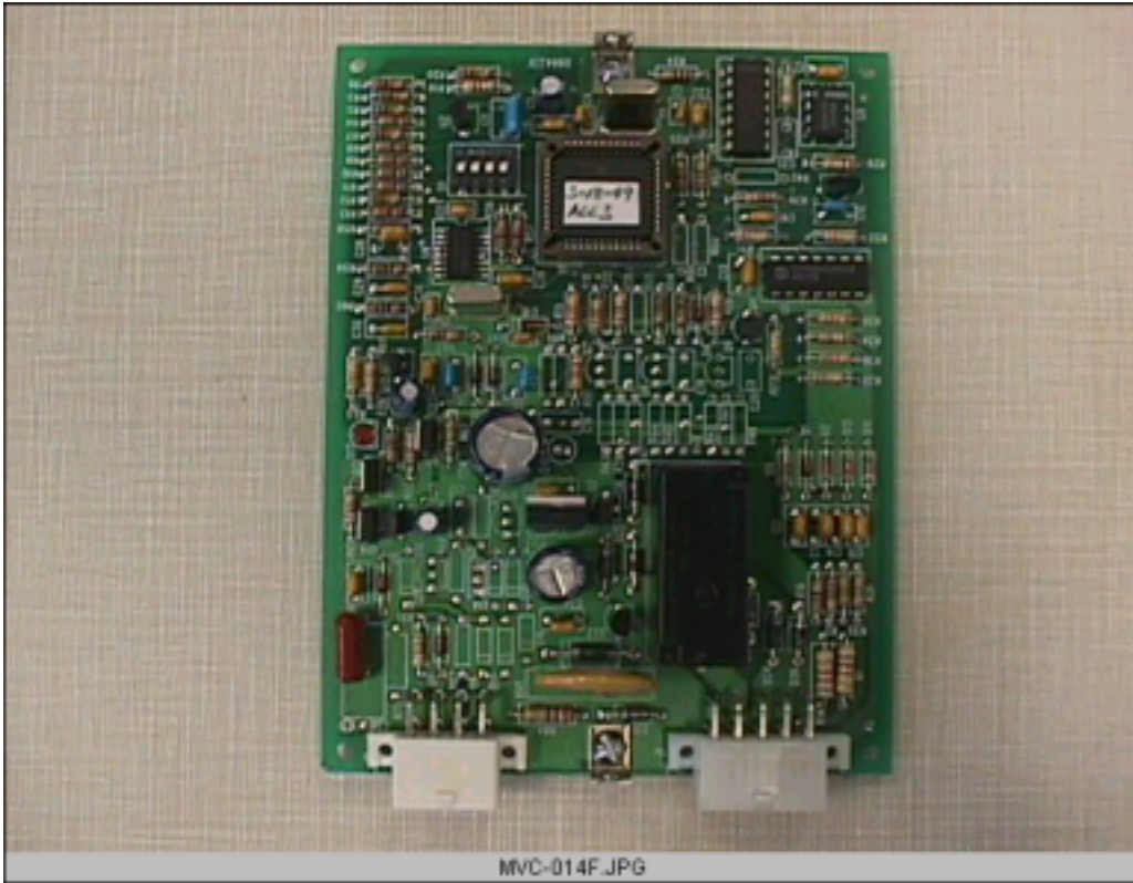
Strattec - Access PCB Board , Close-up
