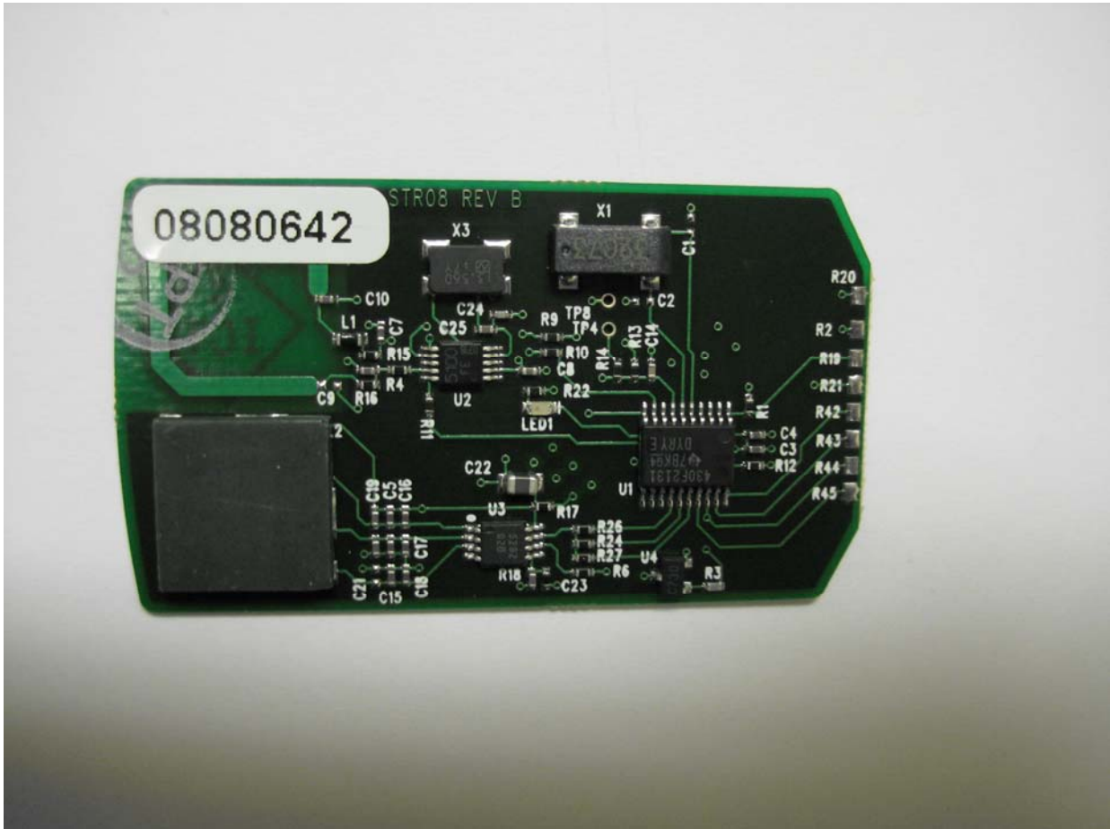
View #1 – Close up of RF Section
